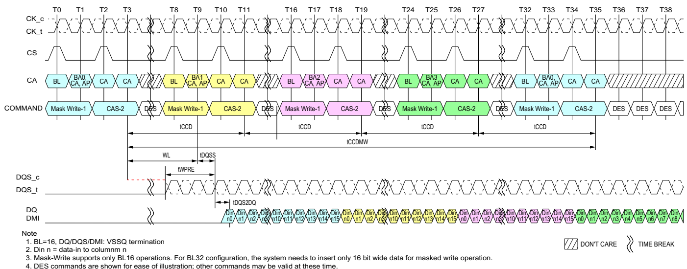
Figure 54 - Masked Write Command - Different Bank
