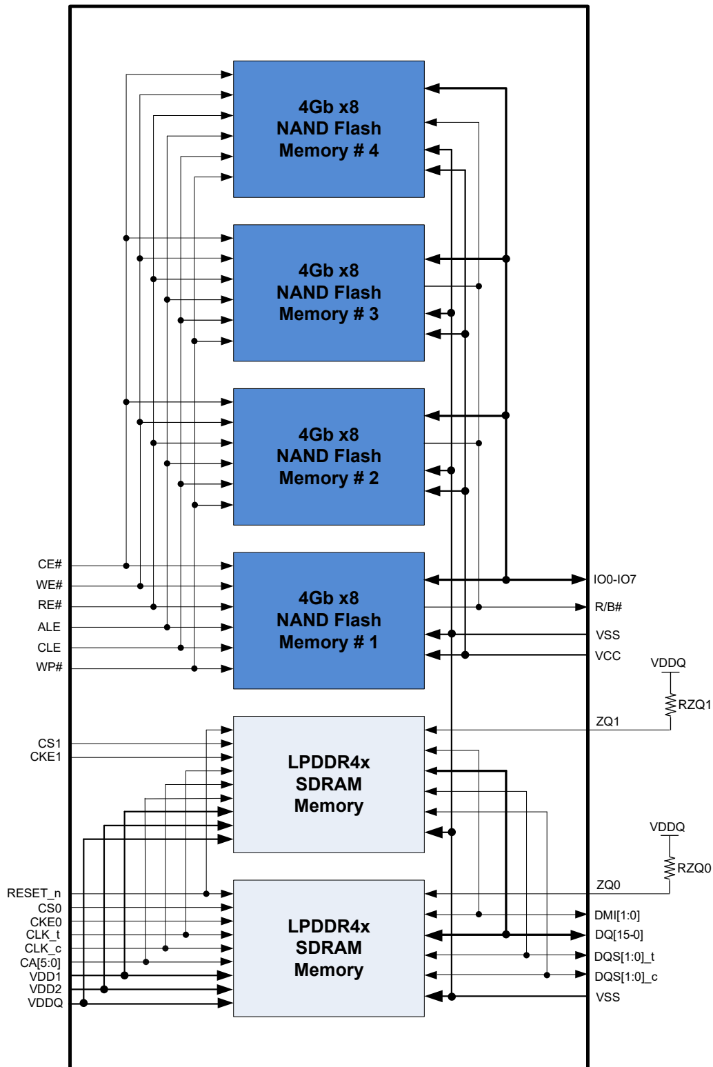
Figure 2.1 Block Diagram
