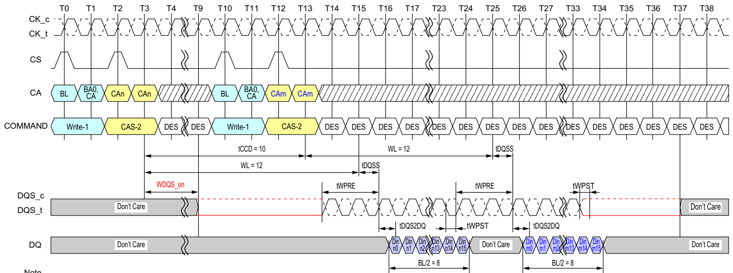
Figure 48 - Consecutive Writes Operation: t_{CCD} = \text{Min} + 2, 0.5n\text{CK} Postamble
