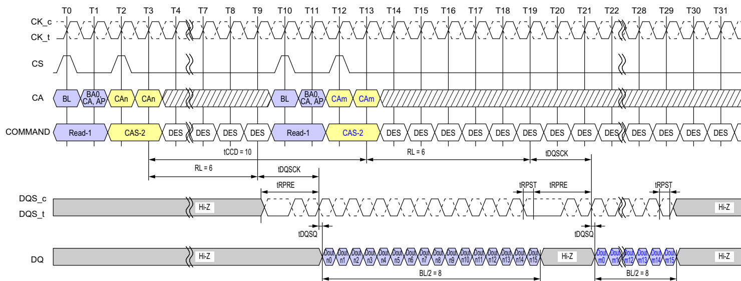
Figure 36 - Consecutive Reads Operation: t_{CCD} = \text{Min} + 2 , Preamble = Toggle, 0.5nCK Postamble
