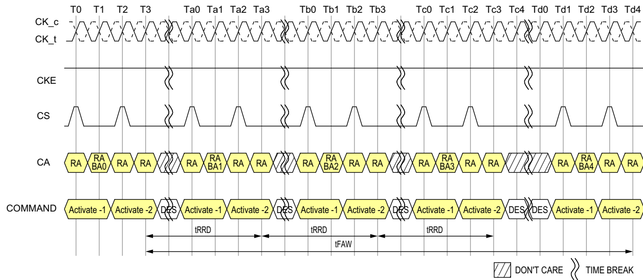
Figure 6 - tFAW Timing
