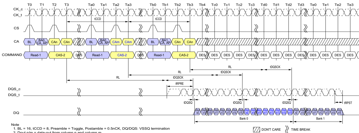
Figure 11 - Seamless Burst Read
