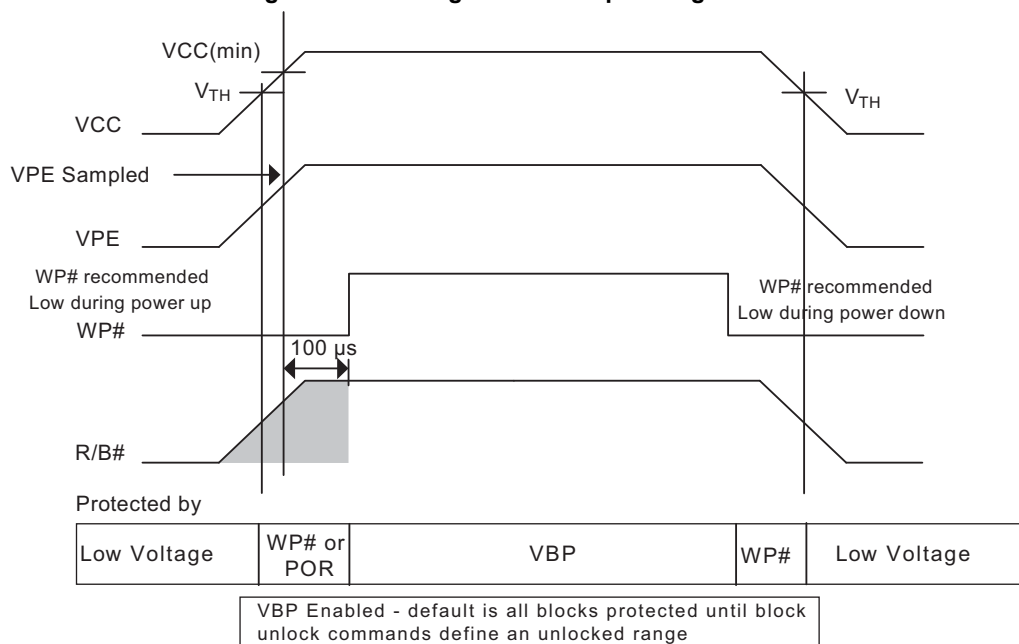
Figure 54. VPE High at Power up Timing [85, 86, 87]
