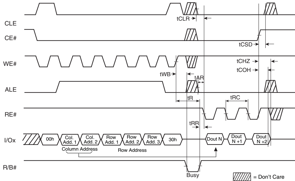
Figure 27. Page Read Operation Interrupted by CE#
