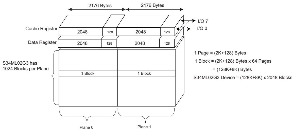
Figure 7. Array Organization — S34ML02G3
