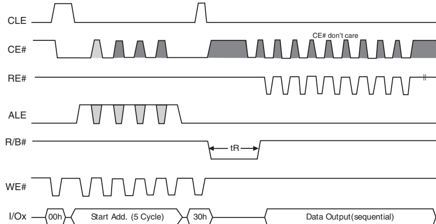
Figure 62. Read Operation with CE# Don't Care
