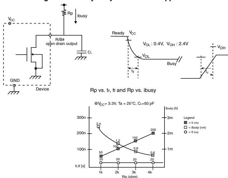
Figure 19. Ready/Busy Pin Electrical Application
