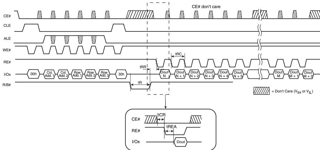
Figure 28. Page Read Operation Timing with CE# Don't Care
