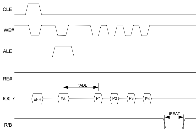
Figure 10. Set Features Timing [18, 19, 20]
