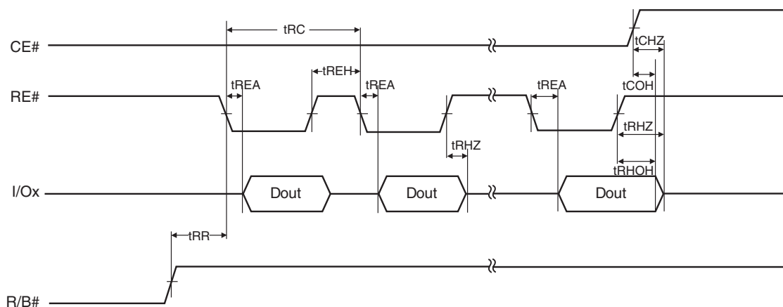
Figure 24. Data Output Cycle Timing [49, 50, 51]
