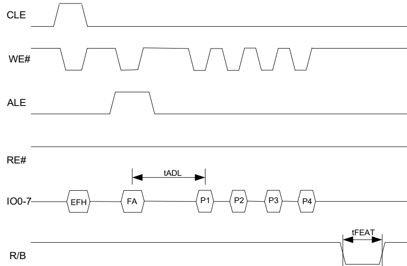
Figure 8. Set Features Timing [18,19,20]
