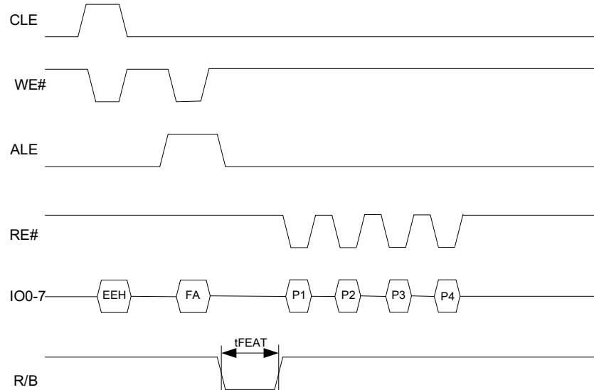
Figure 9. Get Features Timing [23, 24, 25]
