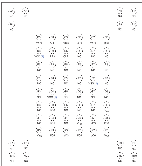
Figure 1.2 63-BGA Contact, x8 Device - 1 CE#, 16Gb (Balls Down, Top View)
