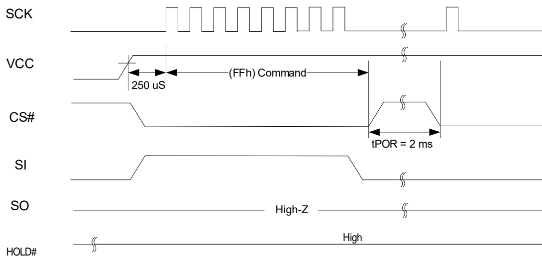
Figure 24. Power Up Timing Diagram (with FFh)
