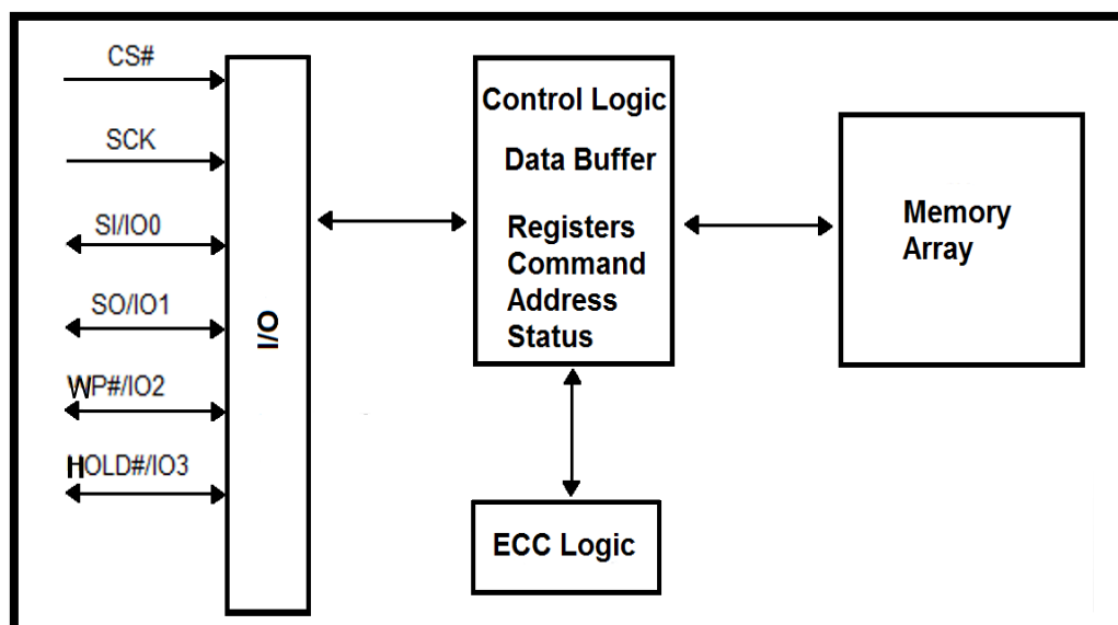
Figure 5. Block Diagram
