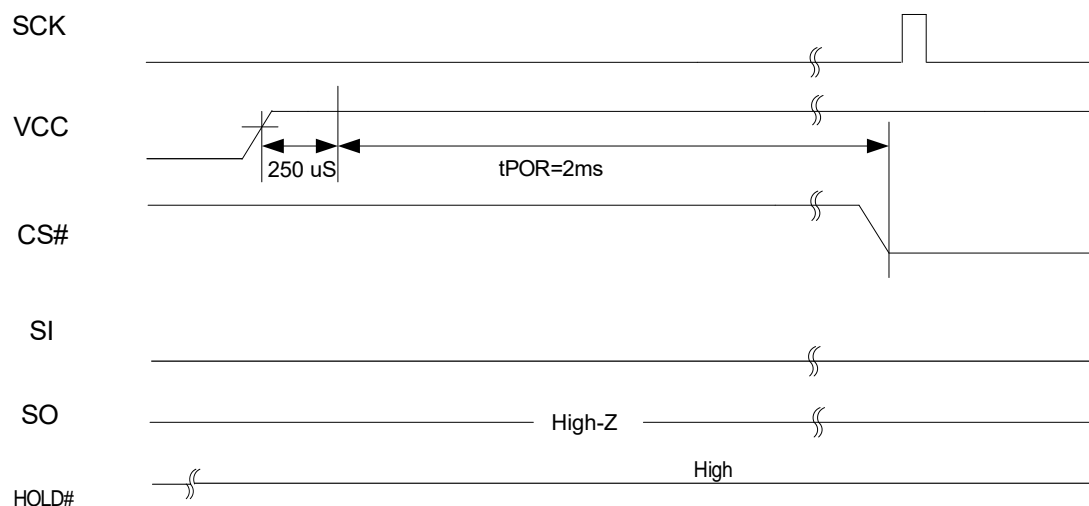
Figure 25. Power up Timing (without FFh)
