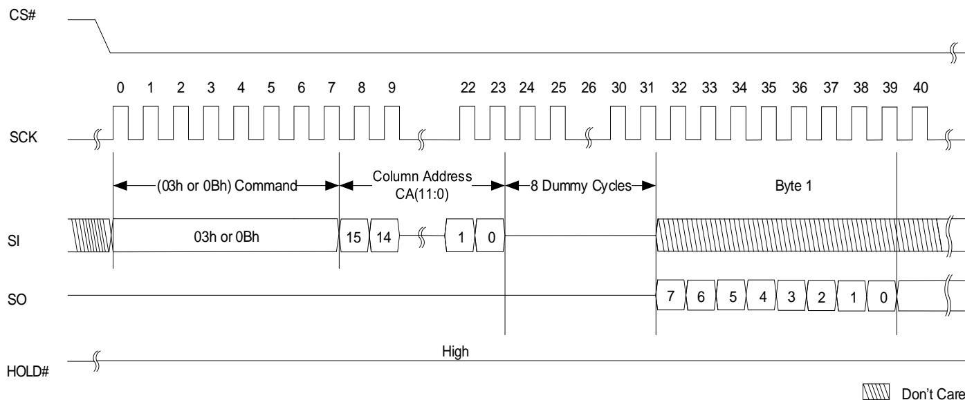
Figure 17: Read Buffer (03h or 0Bh) Timing
