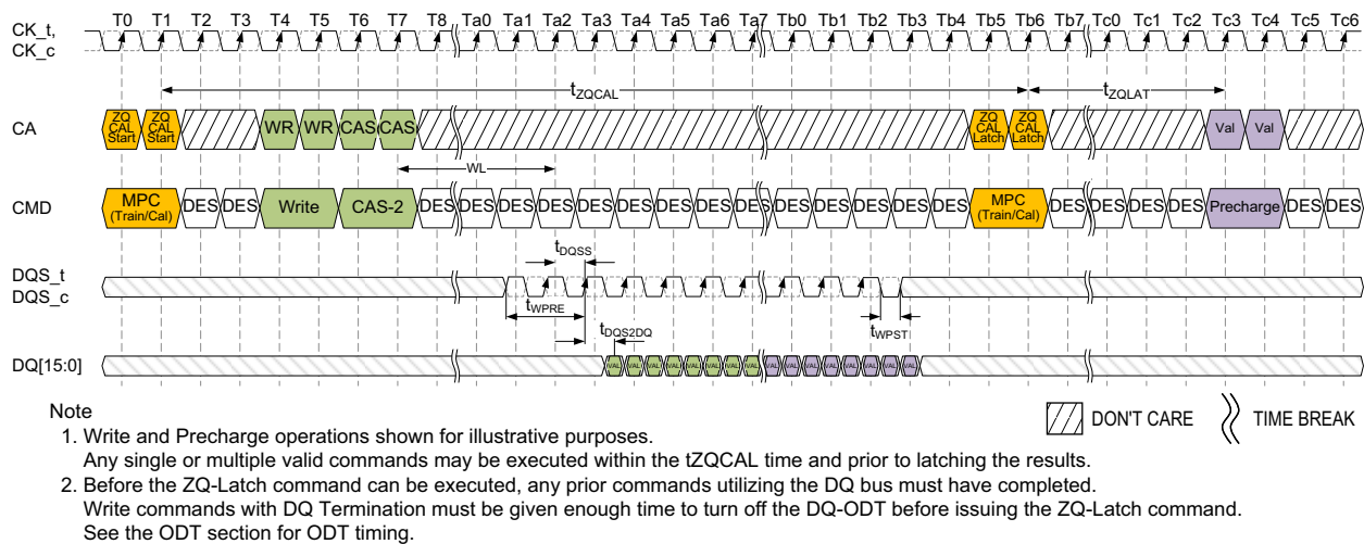
Figure - ZQCal Timing
