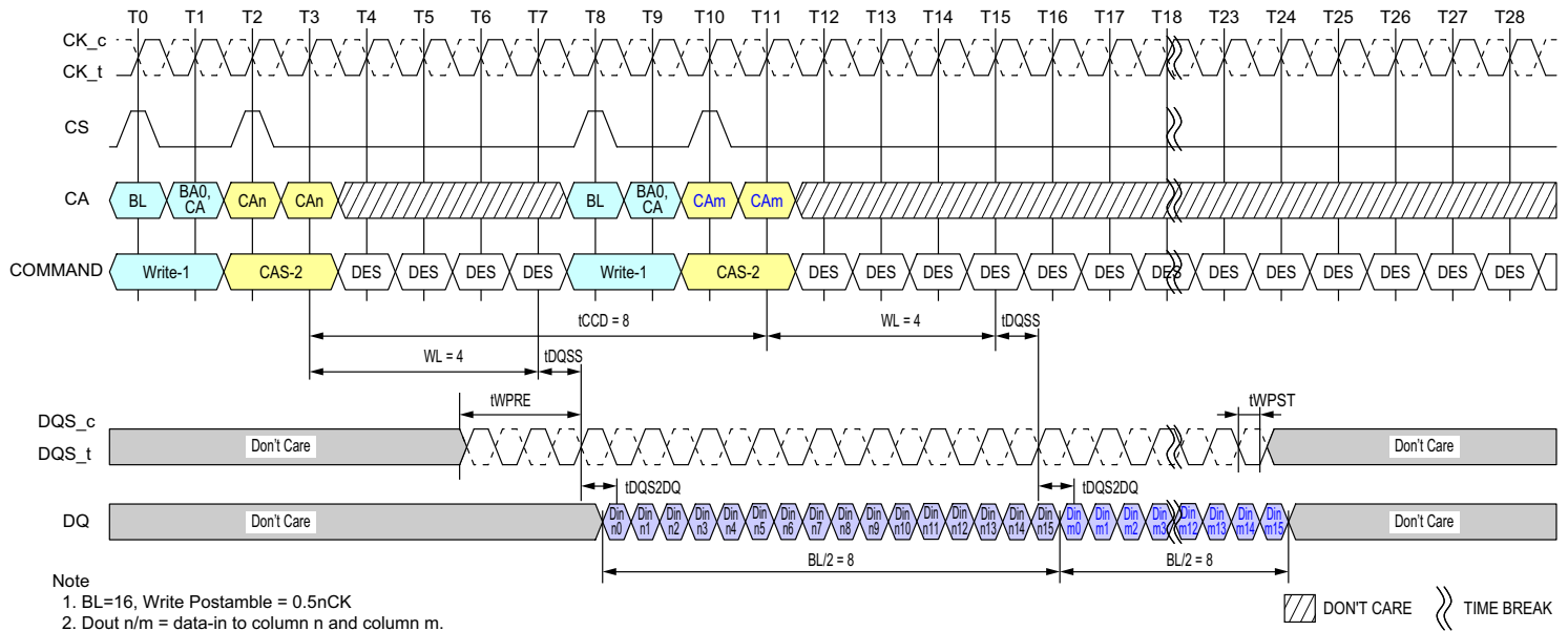
Figure - Seamless Writes Operation: t_{CCD} = \text{Min} , 0.5nCK Postamble
