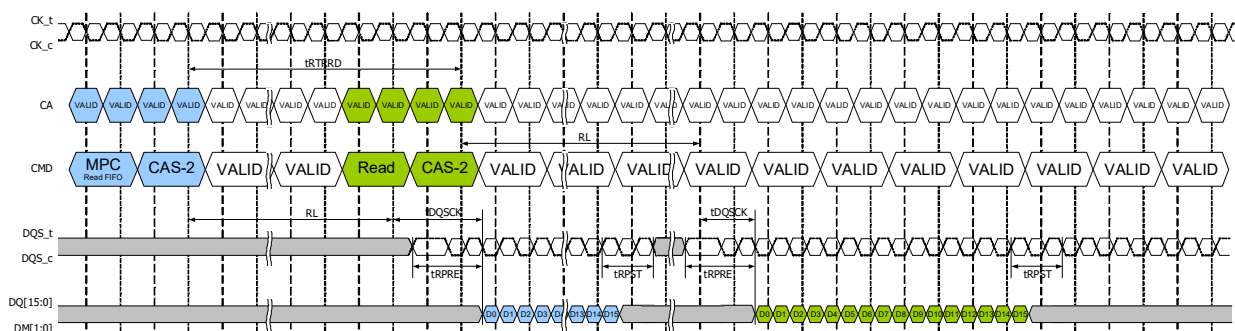
Figure 132 - MPC [RD FIFO] Operation (Shown with tRPRE=toggling, tRPST=1.5nCK)
