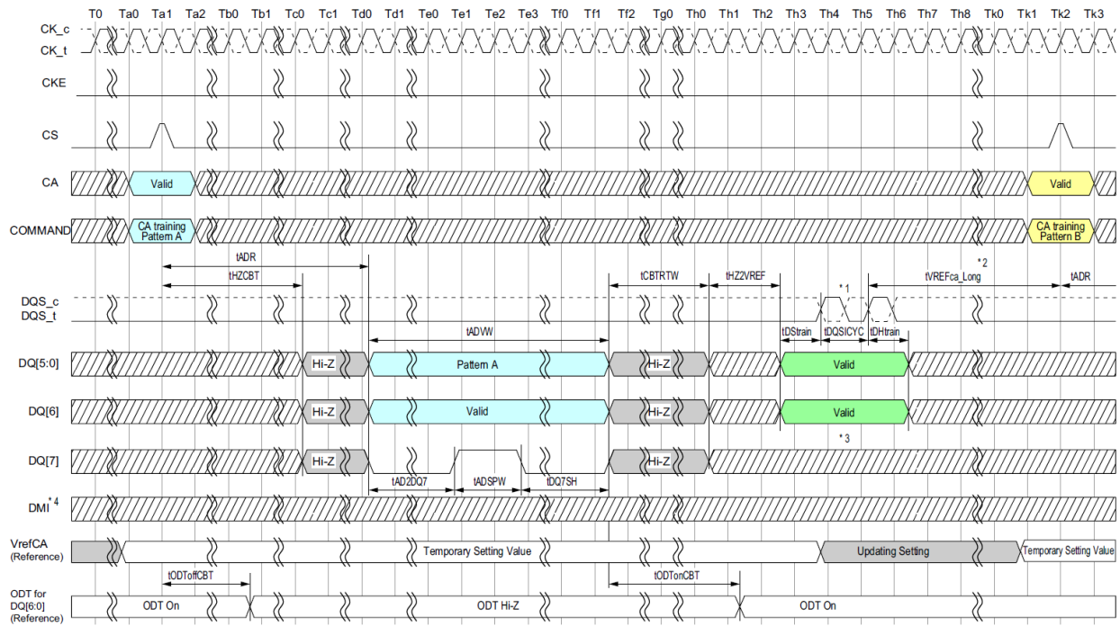
Figure 106 - CA Pattern Input/Output to Vref setting Input
