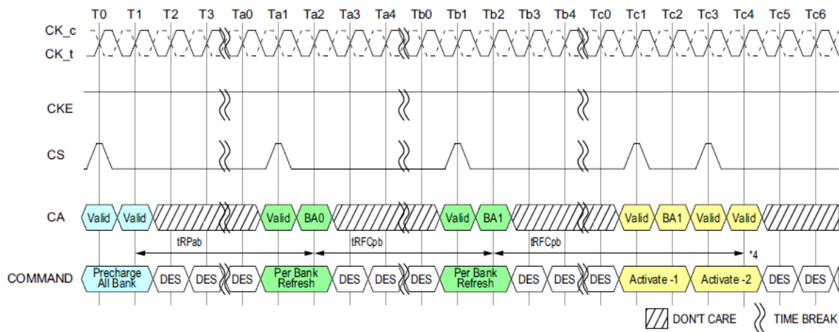
Figure 65 - Per-Bank REFRESH to a different bank Operation
