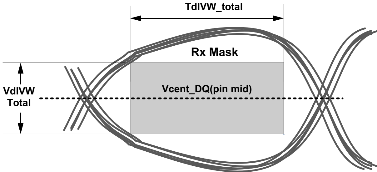
Figure 186 - DQ Receiver(Rx) mask
