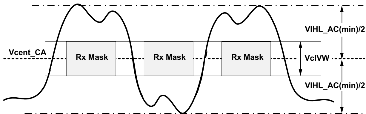
Figure 183 - CA VIHIL_AC definition (for each input pulse)
