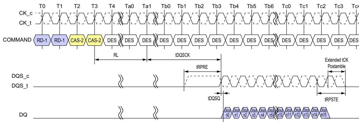
Figure 7 - DQS Read Preamble and Postamble: Static Preamble and 1.5nCK Postamble
