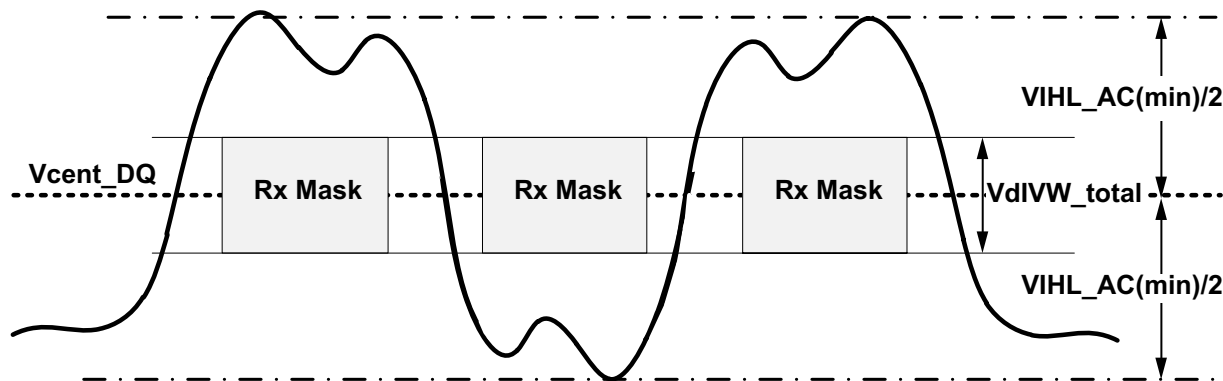
Figure 190 - DQ VIH AC definition (for each input pulse)
