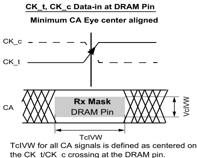
Figure 181 - CA Timing at the DRAM pins
