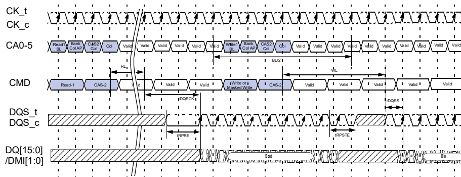
Figure 9 - Burst Read followed by Burst Write. BL=16, Non-toggling tRPRE, Extended tRPSL
