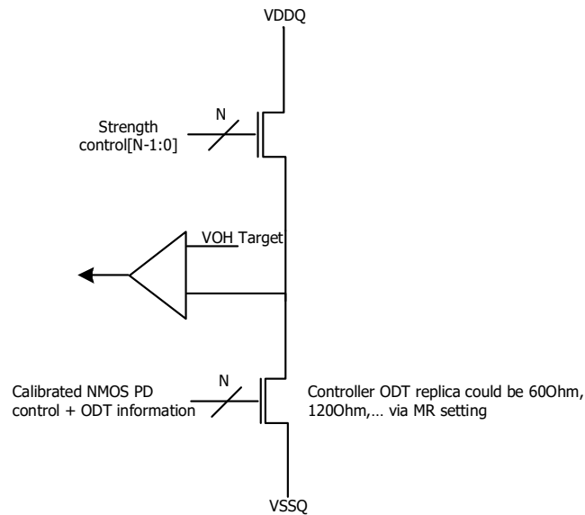
Figure 176 - Pull-up calibration
