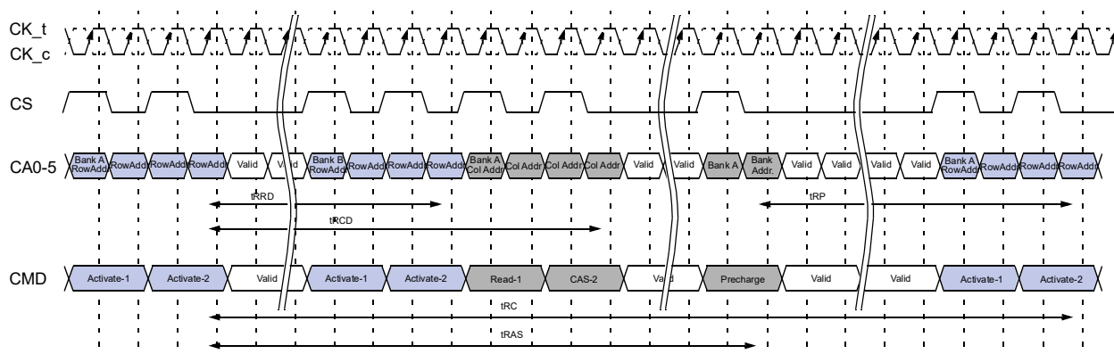
Figure 4 - Activate Command Timing Example
