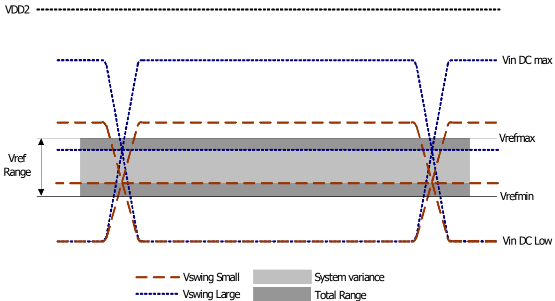
Figure 84 - Vref operating range (Vref.min, Vref.max)
