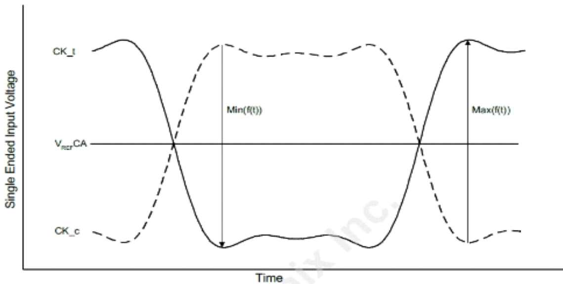
Figure 161 - Definition of differential Clock Peak Voltage
