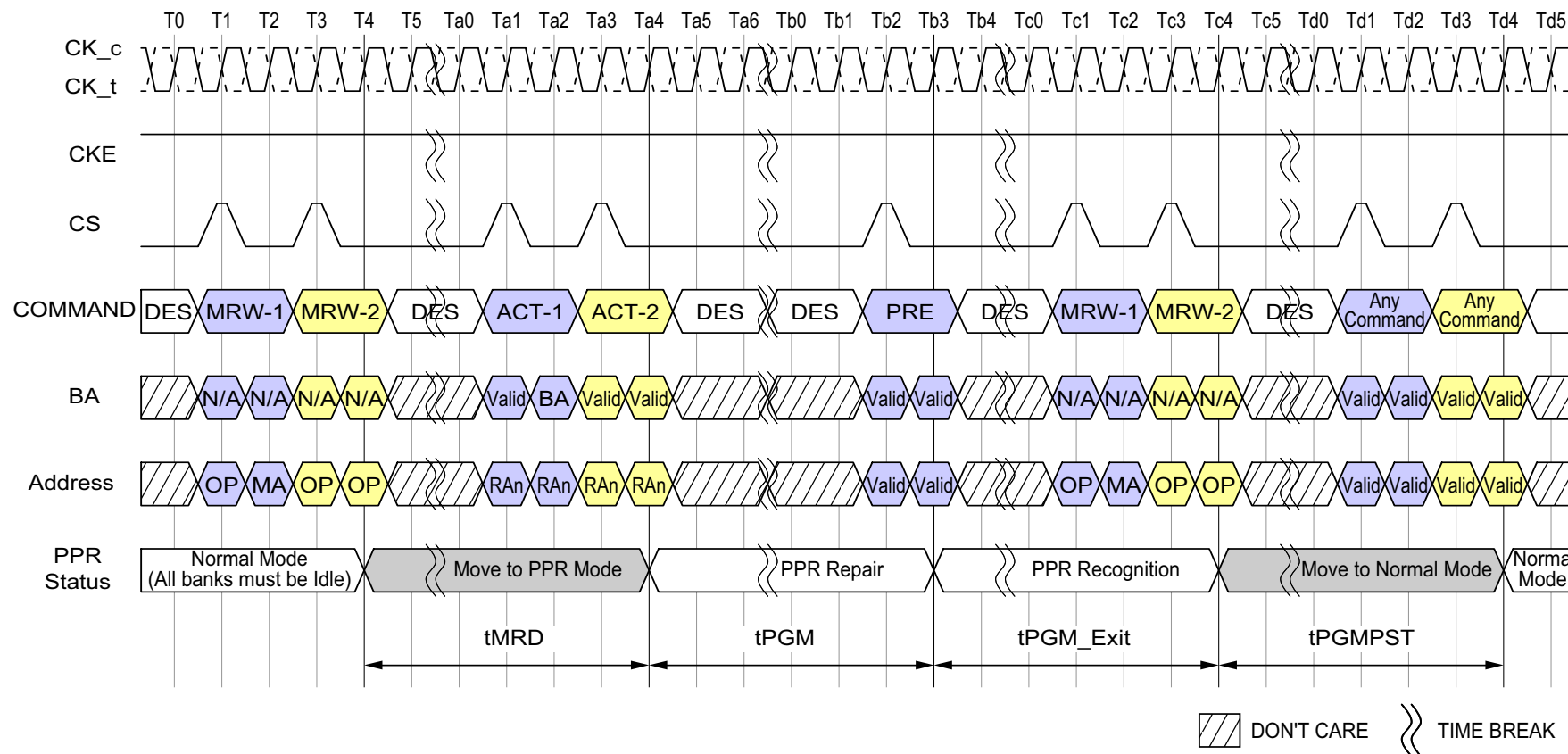
Figure 156 - PPR Timing
