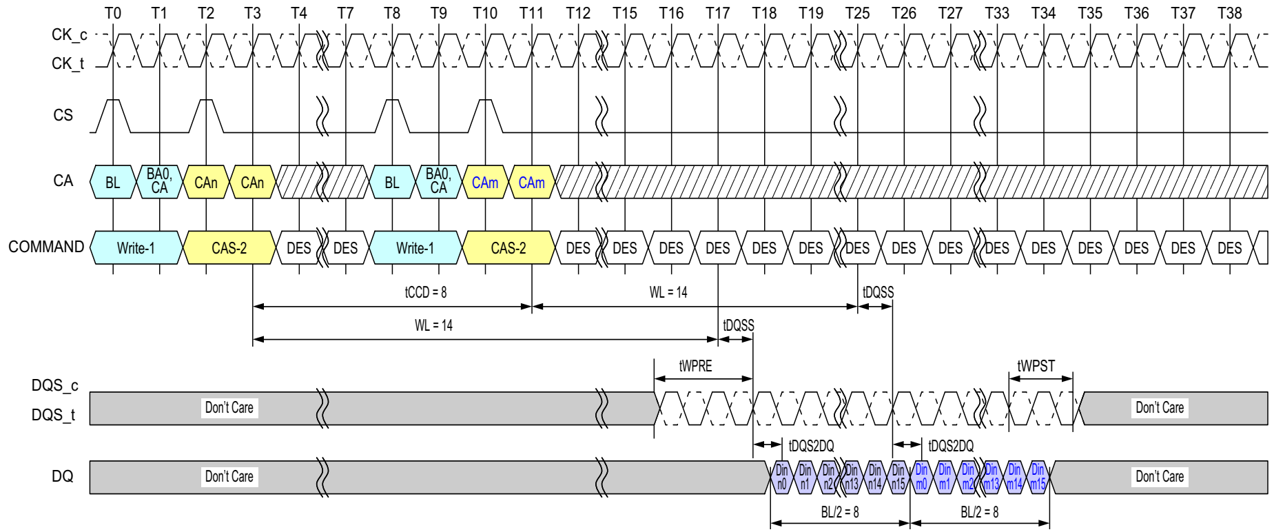
Figure 41 - Seamless Writes Operation: tCCD = Min, 1.5nCK Postamble
