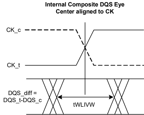
Figure 177 - DQS_t/DQS_c and CK_t/CK_c at DRAM Latch
