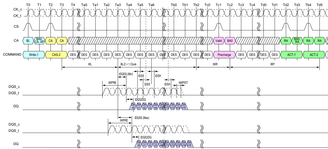
Figure 21 - Burst Write Operation
