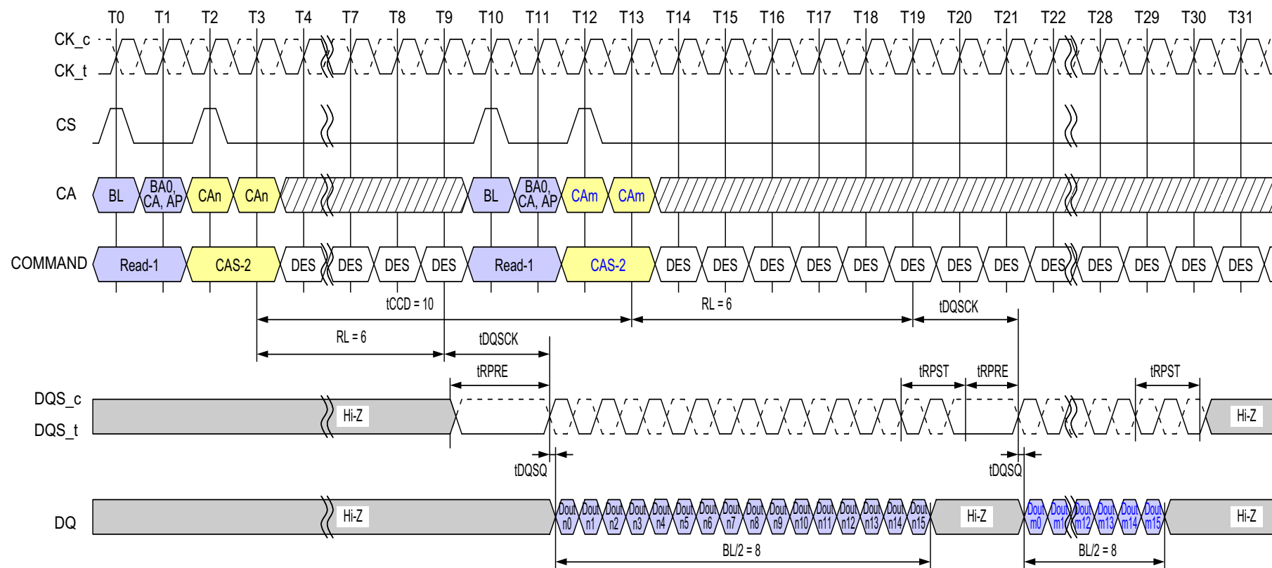
Figure 33 - Consecutive Reads Operation: tCCD = Min +2, Preamble = Static, 1.5nCK Postamble
