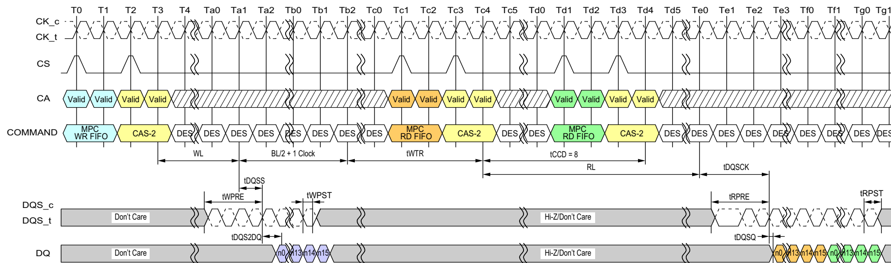
Figure 122 - MPC [Write FIFO] to MPC [Read FIFO] Timing
