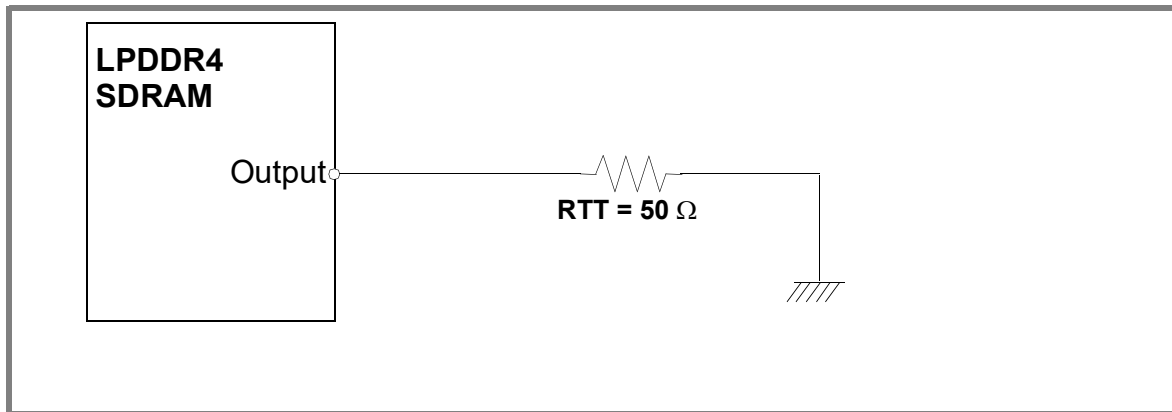
Figure 173 - Driver Output Reference Load for Timing and Slew Rate
