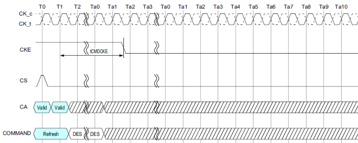
Figure 149 - Refresh entry to Power-Down Entry
