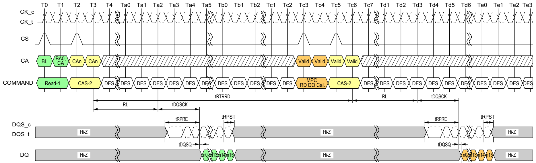
Figure 118 - DQ Read Training Timing: Read to Read DQ Calibration
