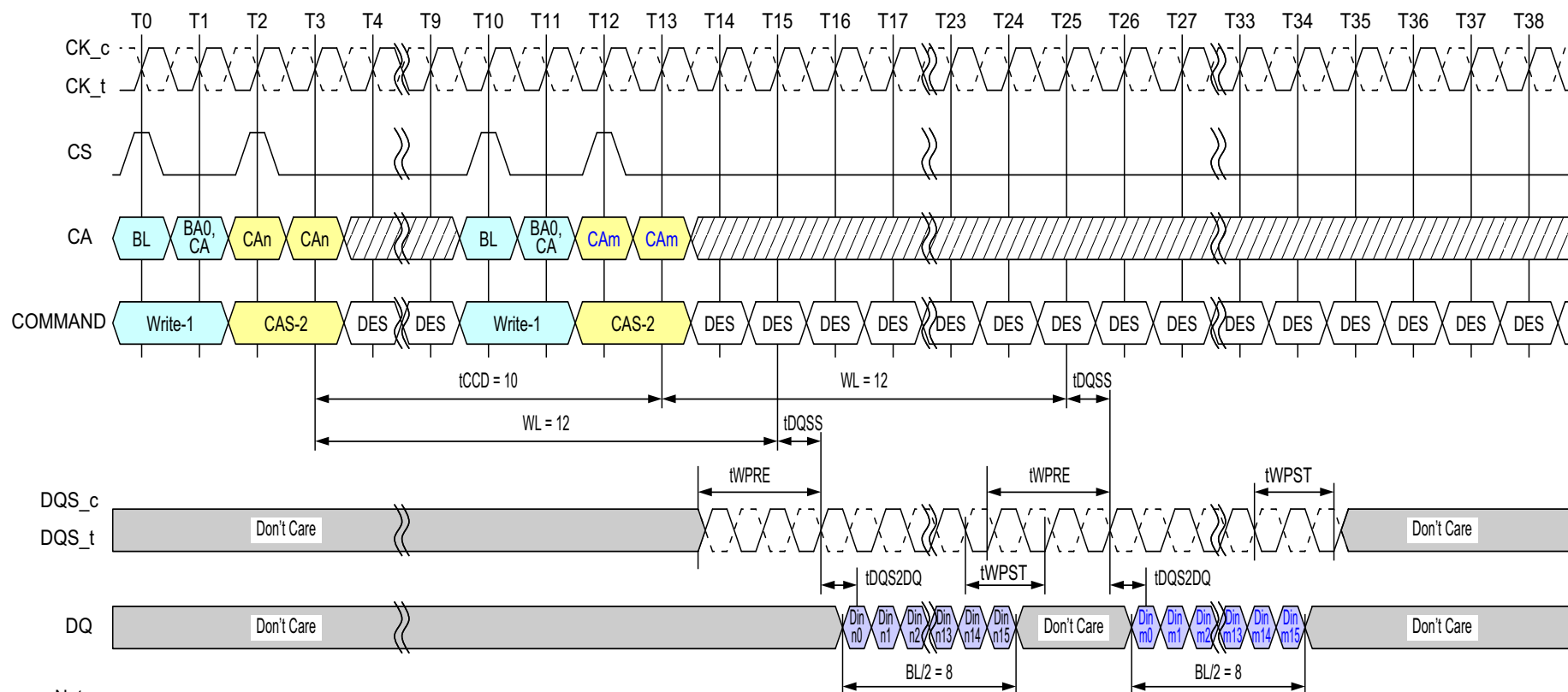
Figure 45 - Consecutive Writes Operation: t_{CCD} = \text{Min} + 2, 1.5nCK Postamble
