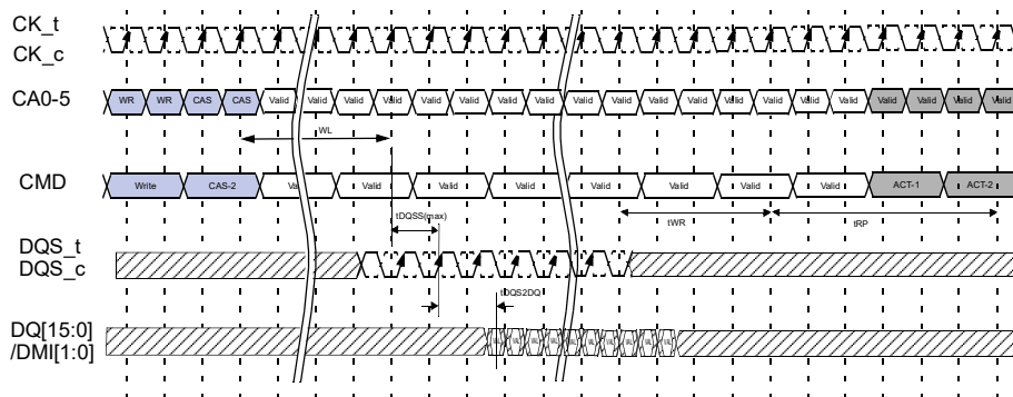
Figure 59 - Burst Write with Auto-Precharge (BL16, 2tCK preamble)
