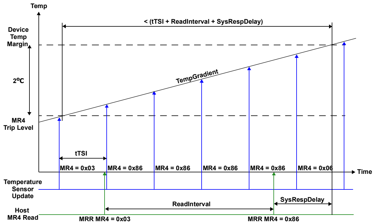
Figure 133 - Temp sensor Timing
