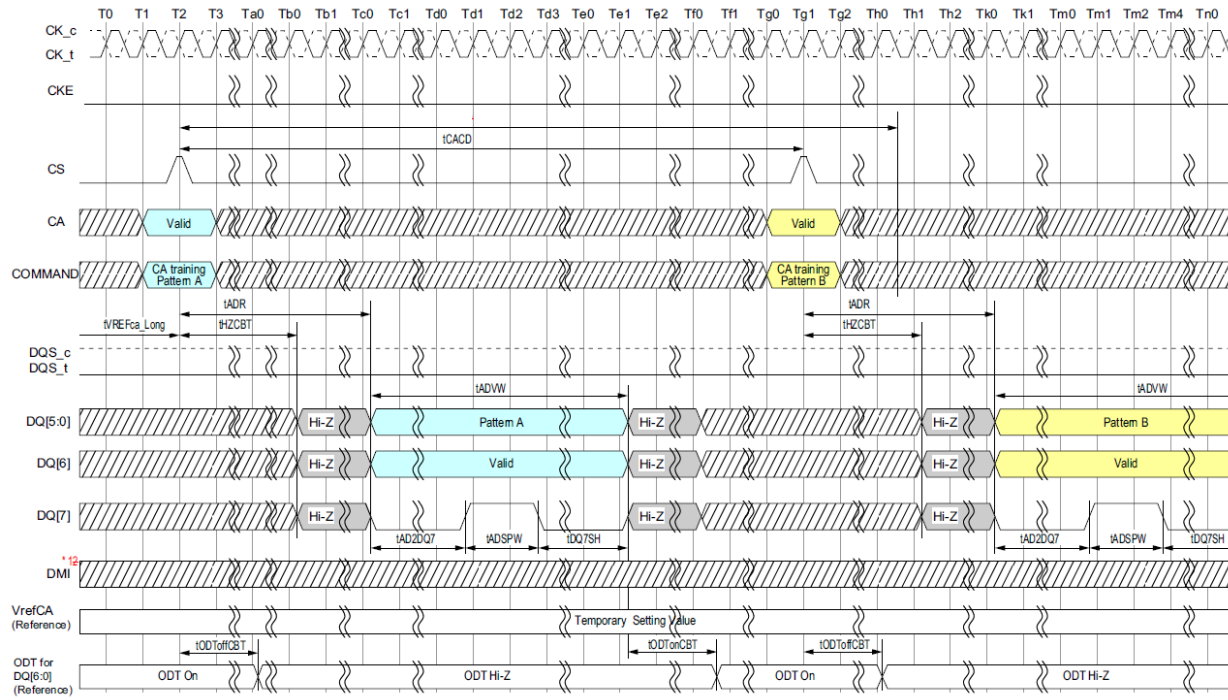
Figure 107 - Consecutive CA Training pattern Input/Output
