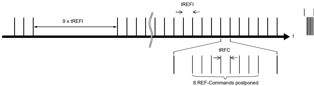
Figure 67 - Postponing Refresh Commands (Example)
