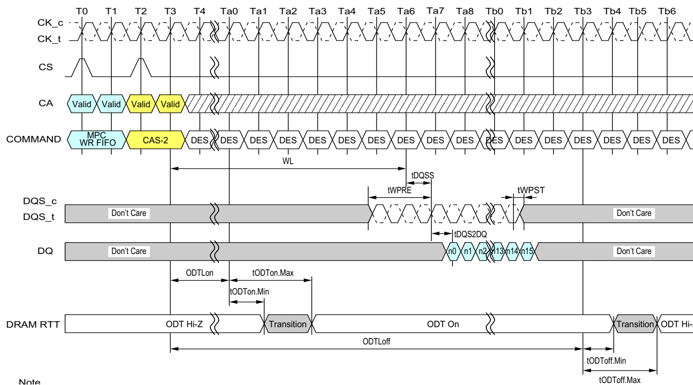
Figure 124 - MPC [Write FIFO] with DQ ODT Timing
