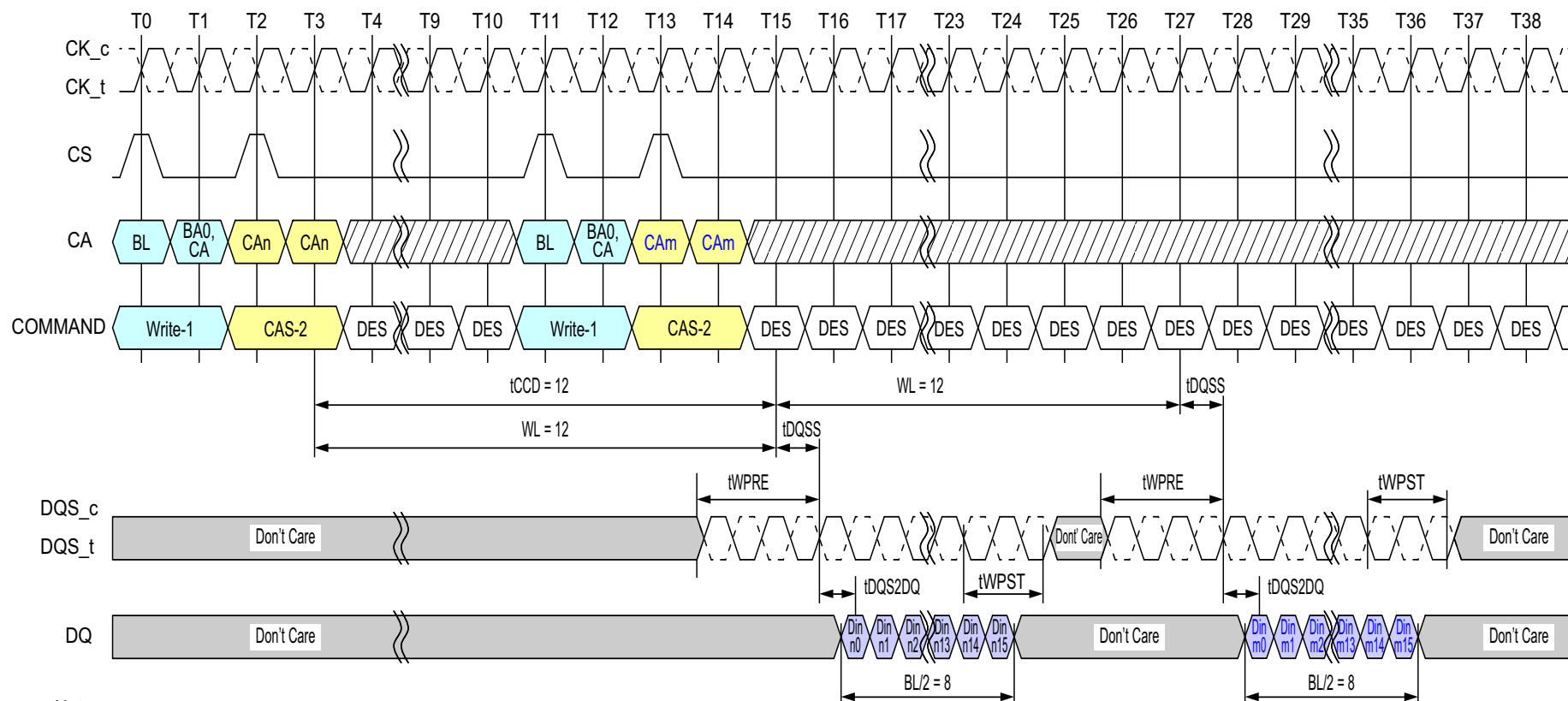
Figure 48 - Consecutive Writes Operation: t_{CCD} = \text{Min} + 4, 1.5nCK Postamble
