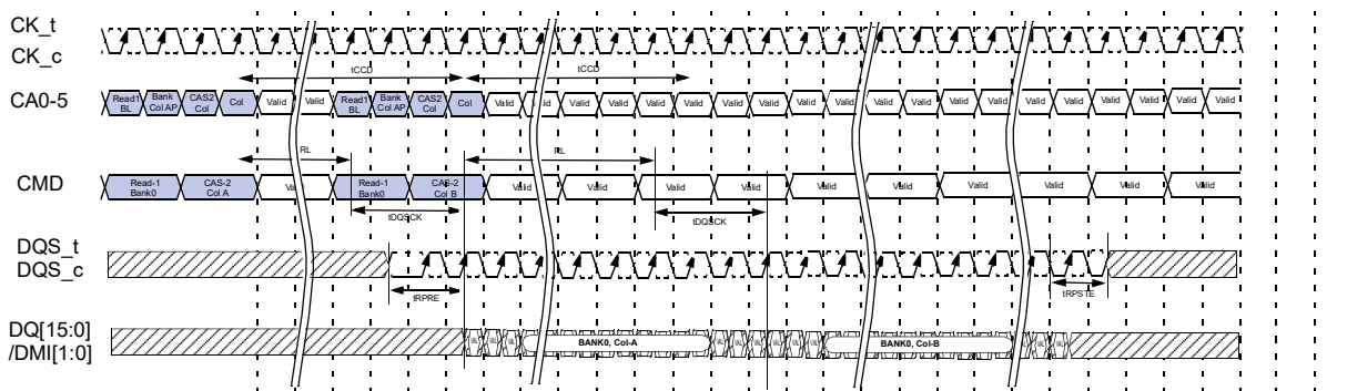
Figure 8 - Burst Read Timing. BL=16, Toggling tRPRE, Extended tRPSL
