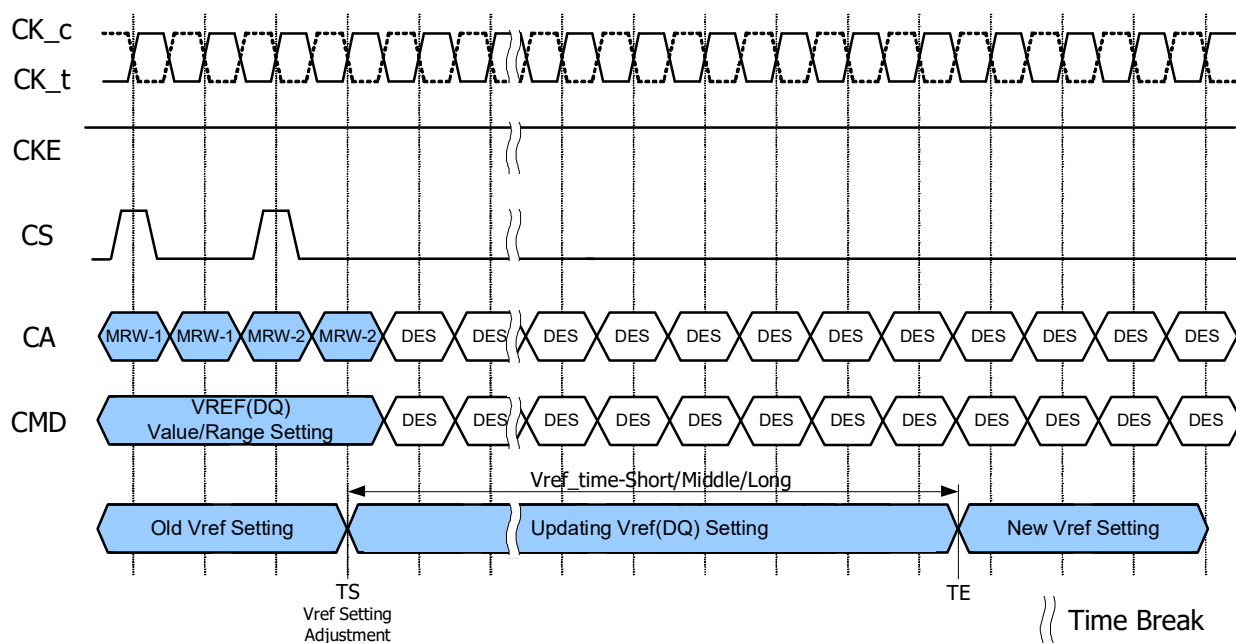
Figure 93 - Vref_time for short and long timing diagram
