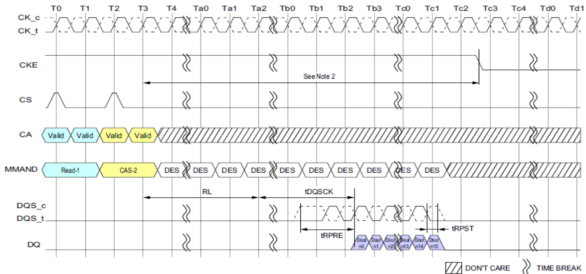
Figure 146 - Read and Read with Auto-precharge to Power-Down Entry
