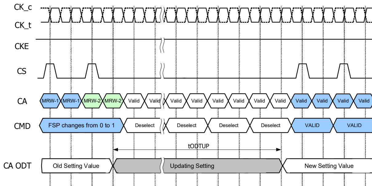
Figure 139 - CA ODT setting update timing in 4 Clock Cycle Command
