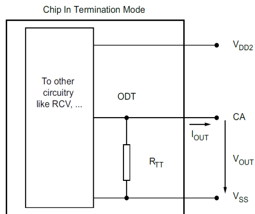
Figure 137 - CA On Die Termination
