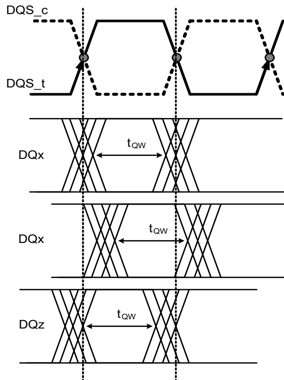
Figure 185 - Read data timing t_{QW} valid window defined per DQ signal
