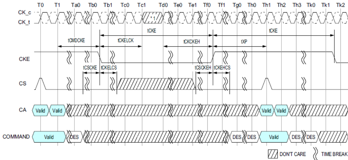
Figure 145 - Basic Power-down Entry and Exit Timing
