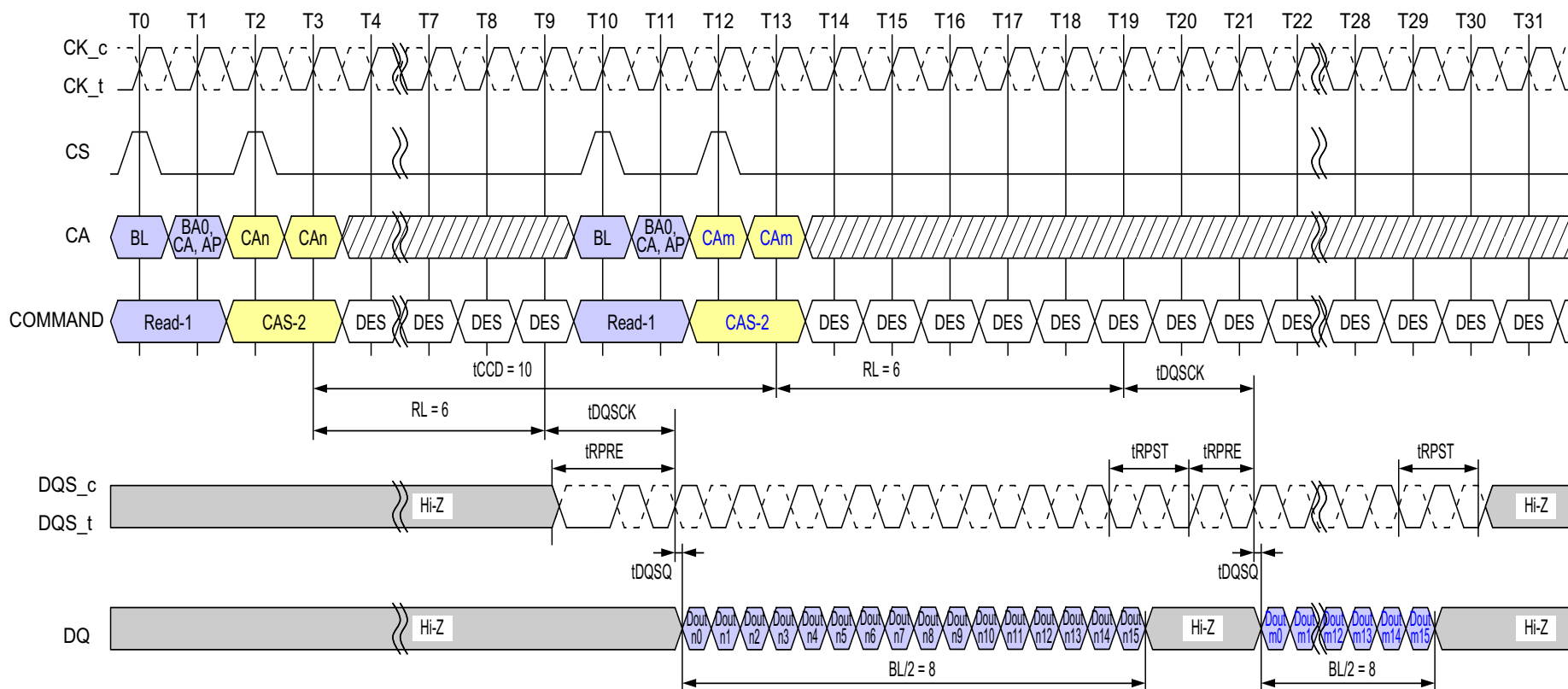
Figure 31 - Consecutive Reads Operation: t_{CCD} = \text{Min} + 2 , Preamble = Toggle, 1.5nCK Postamble
