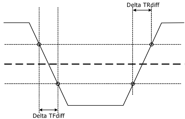
Figure 171 - Differential Output Slew Rate Definition
