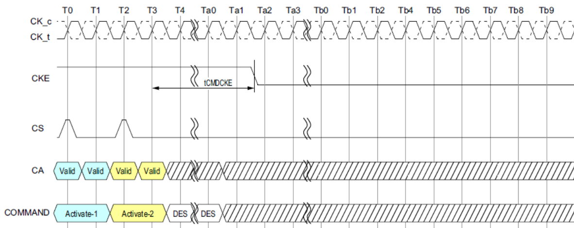
Figure 150 - Activate Command to Power-Down Entry
