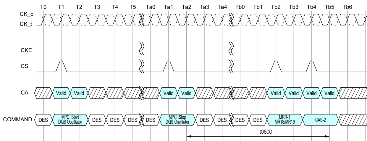
Figure 127 - In case of DQS Interval Oscillator is stopped by MPC Command
