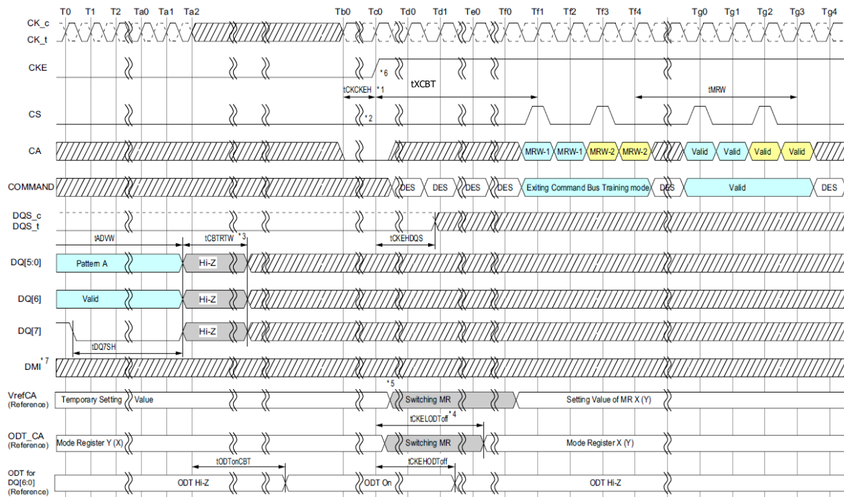
Figure 108 - Exiting Command Bus Training Mode 2
