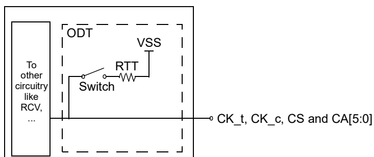
Figure 136 - Functional Representation of CA ODT
