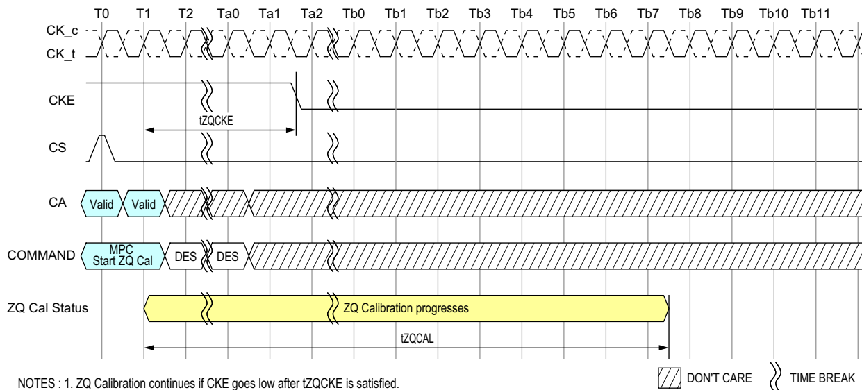
Figure 154 - MPC ZQCAL_start to Power-Down Entry
