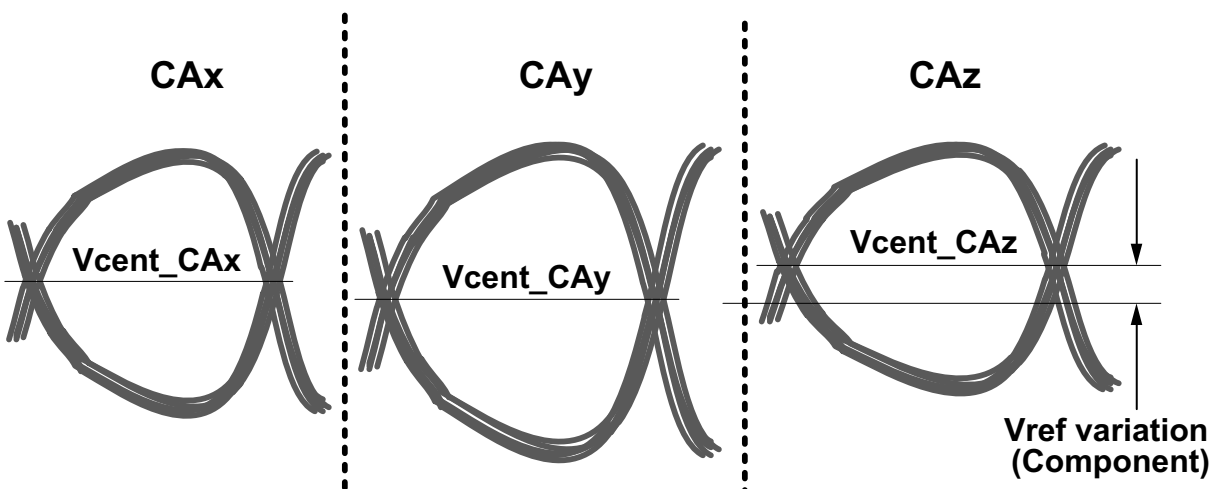
Figure 180 - Across pin Vref CA voltage variation
