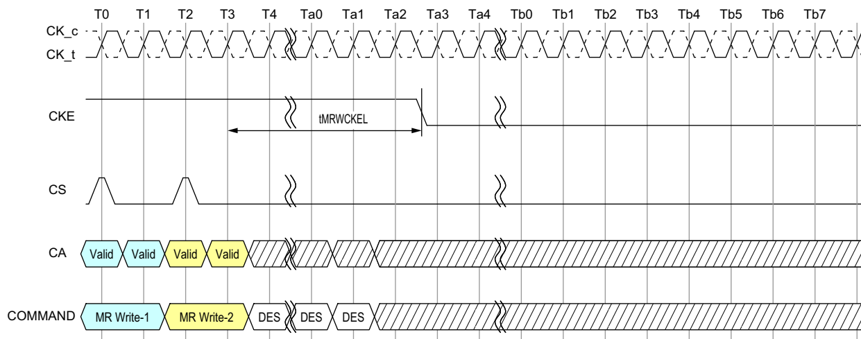
Figure 153 - MRW to Power-Down Entry
