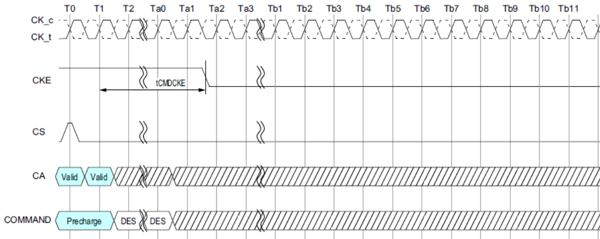
Figure 151 - Precharge Command to Power-Down Entry
