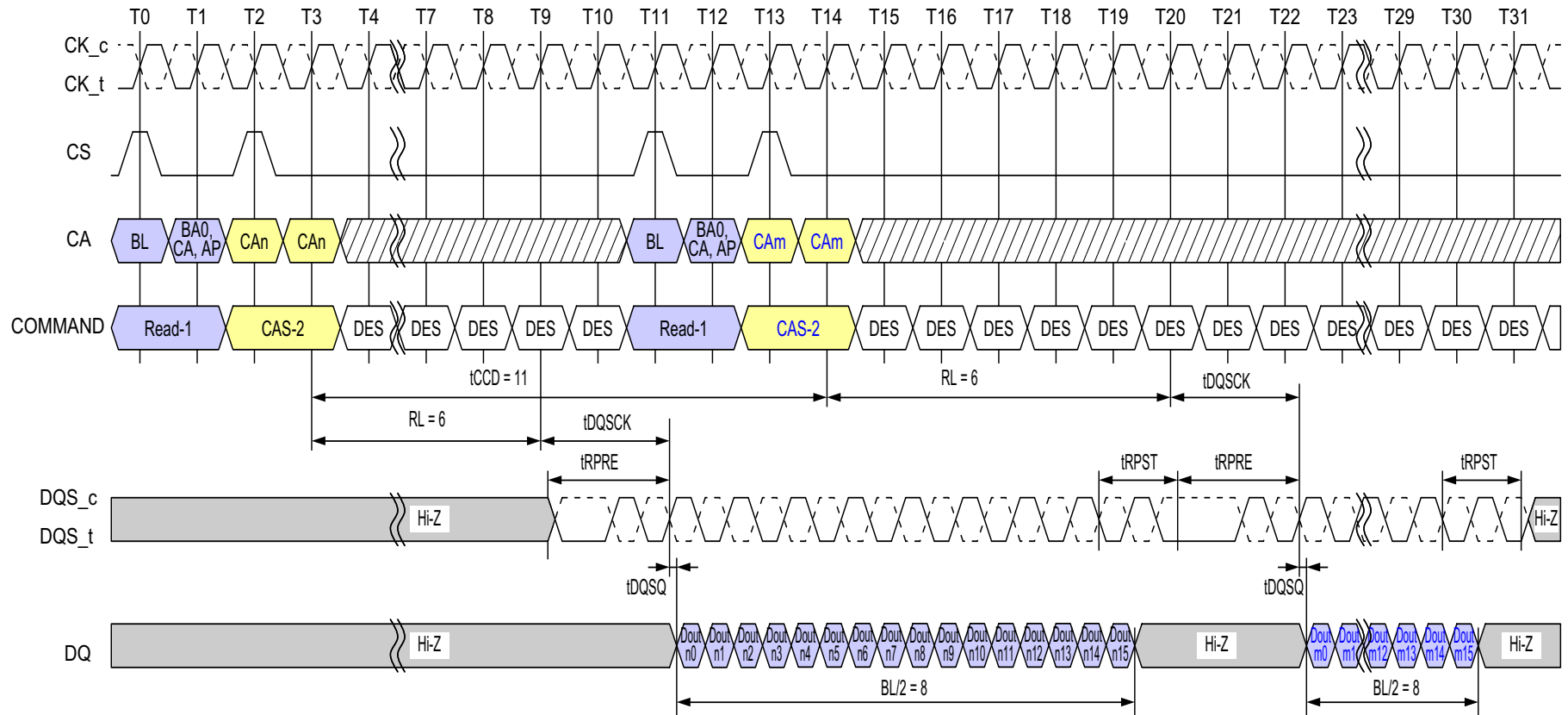
Figure 35 - Consecutive Reads Operation: tCCD = Min +3, Preamble = Toggle, 1.5nCK Postamble
