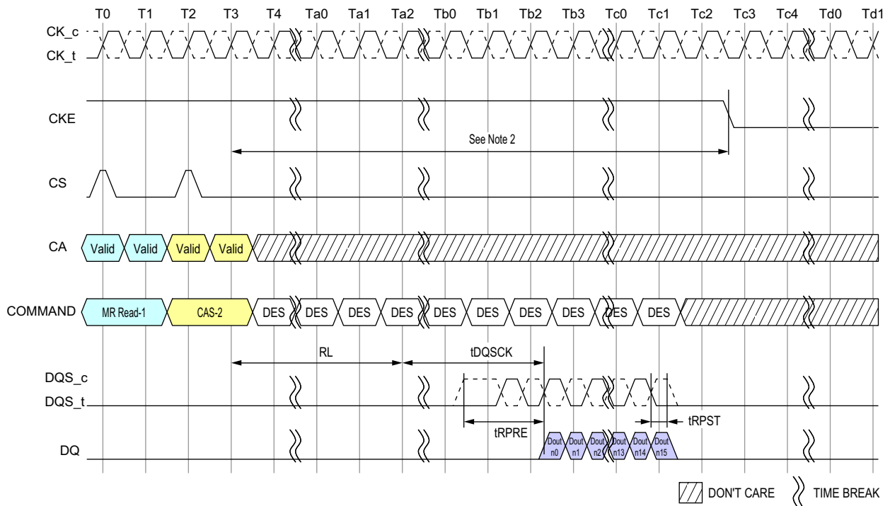
Figure 152 - Mode Register Read to Power-Down Entry
