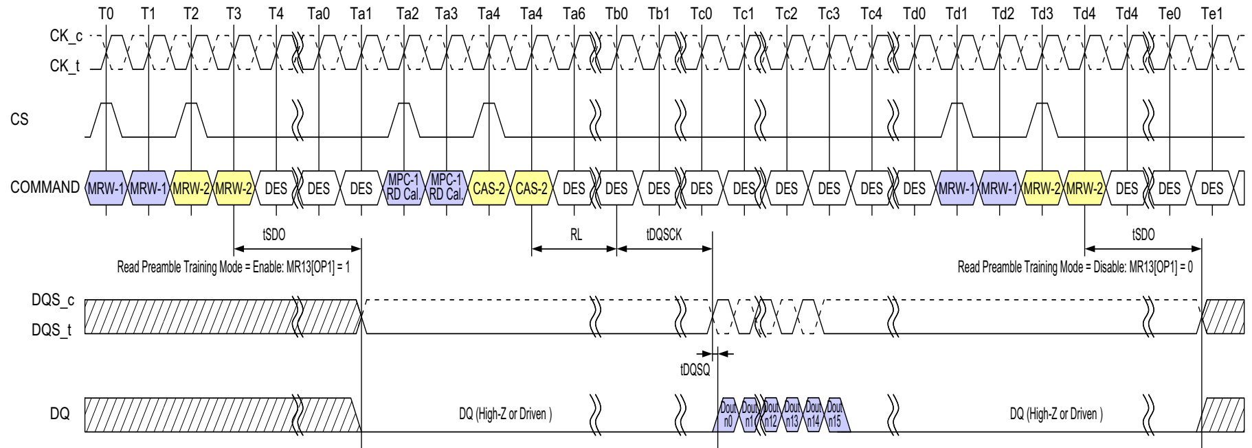
Figure 129 - Read Preamble Training
