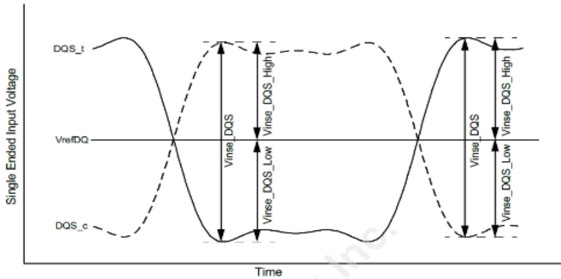
Figure 167 - DQS Single-Ended Input Voltage
