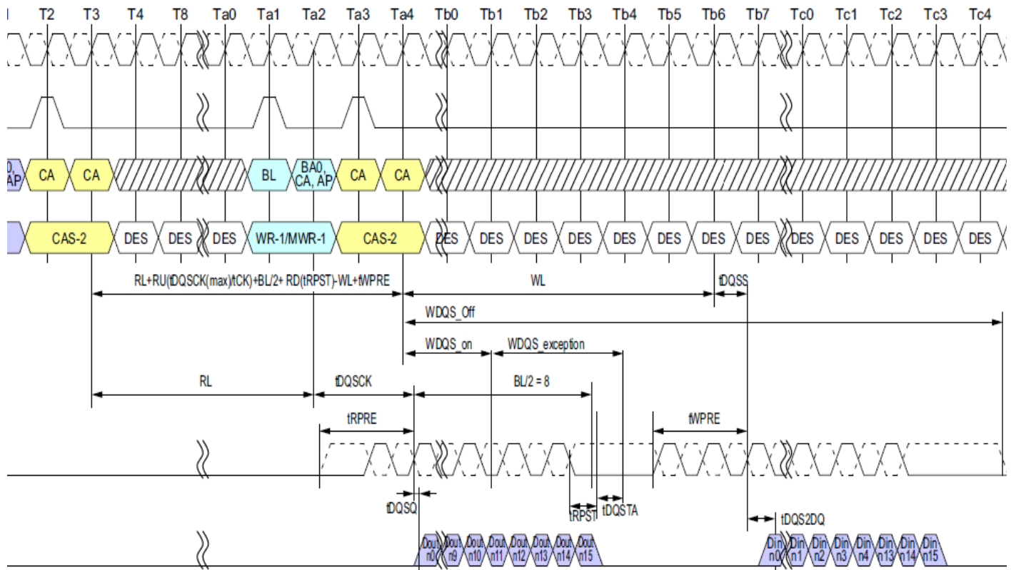
Figure 62 - Burst Read followed by Burst Write or Burst Mask Write (ODT Disable)
