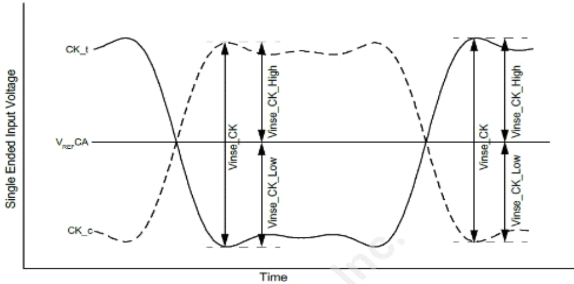
Figure 162 - Clock Single-Ended Input Voltage
