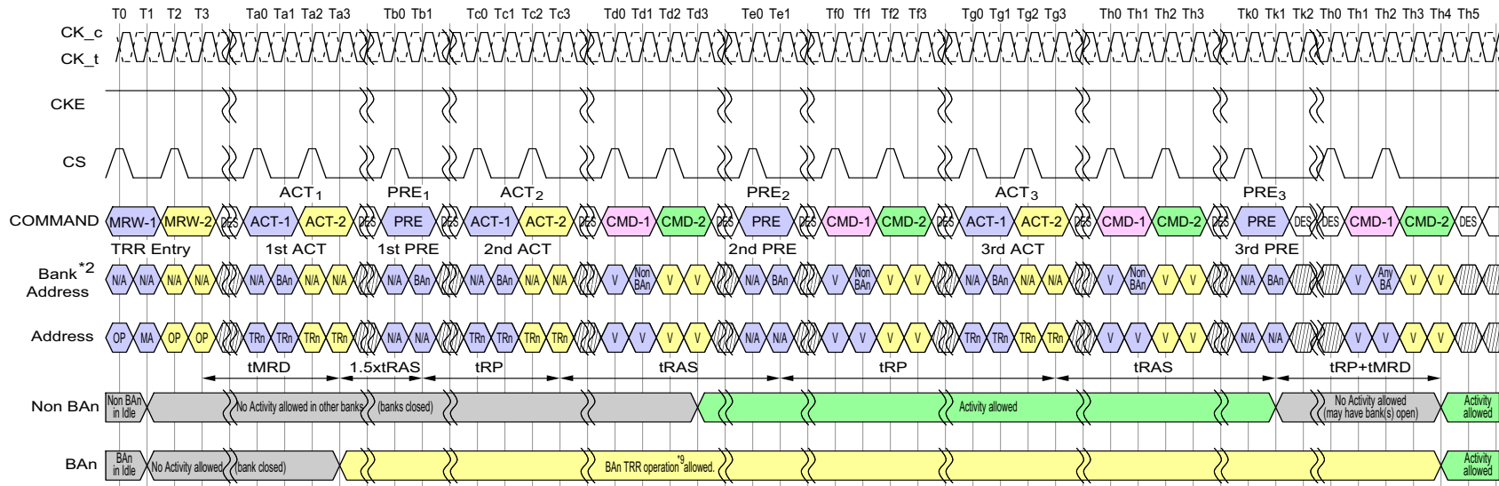
Figure 155 - TRR Mode Timing Example
