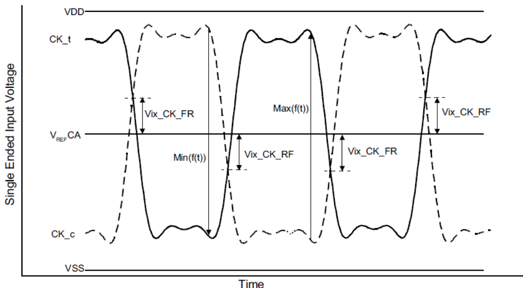
Figure 164 - Vix Definition (Clock)
