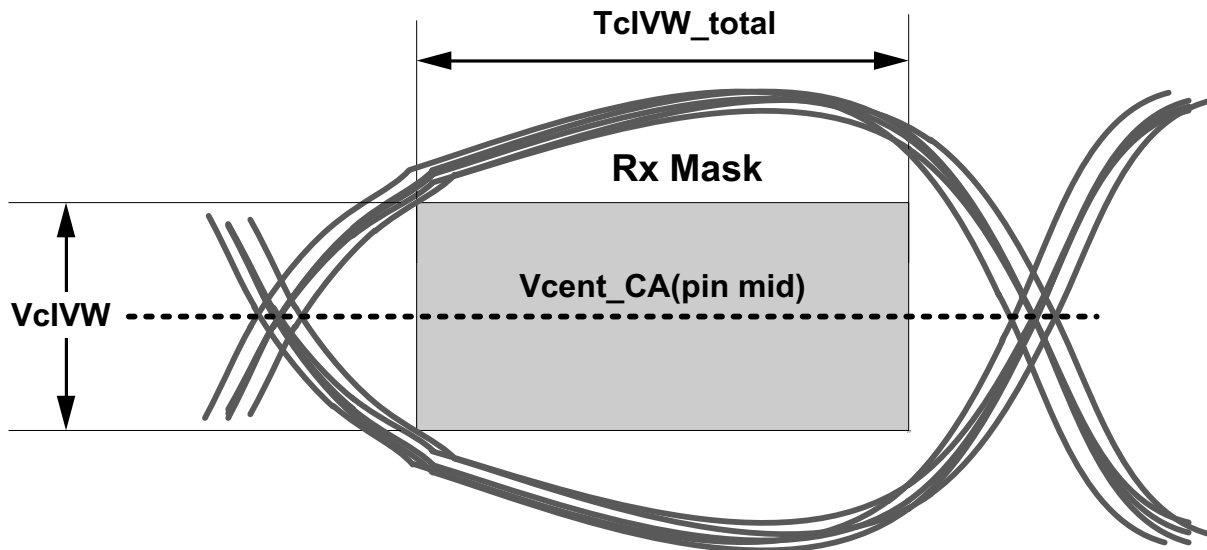
Figure 179 - CA Receiver(Rx) mask
