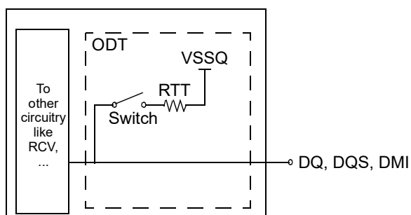
Figure 140 - Functional Representation of ODT
