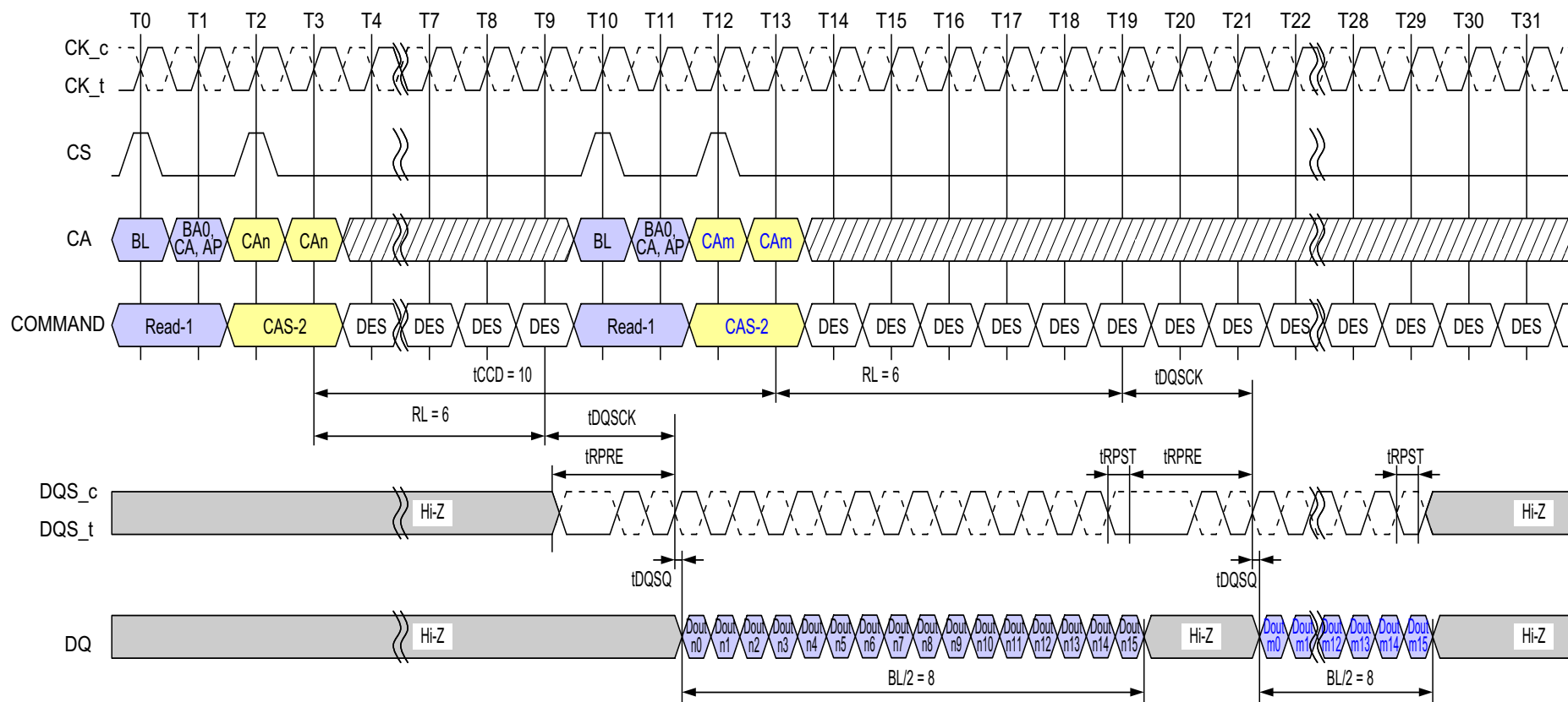
Figure 32 - Consecutive Reads Operation: t_{CCD} = \text{Min} + 2 , Preamble = Toggle, 0.5nCK Postamble
