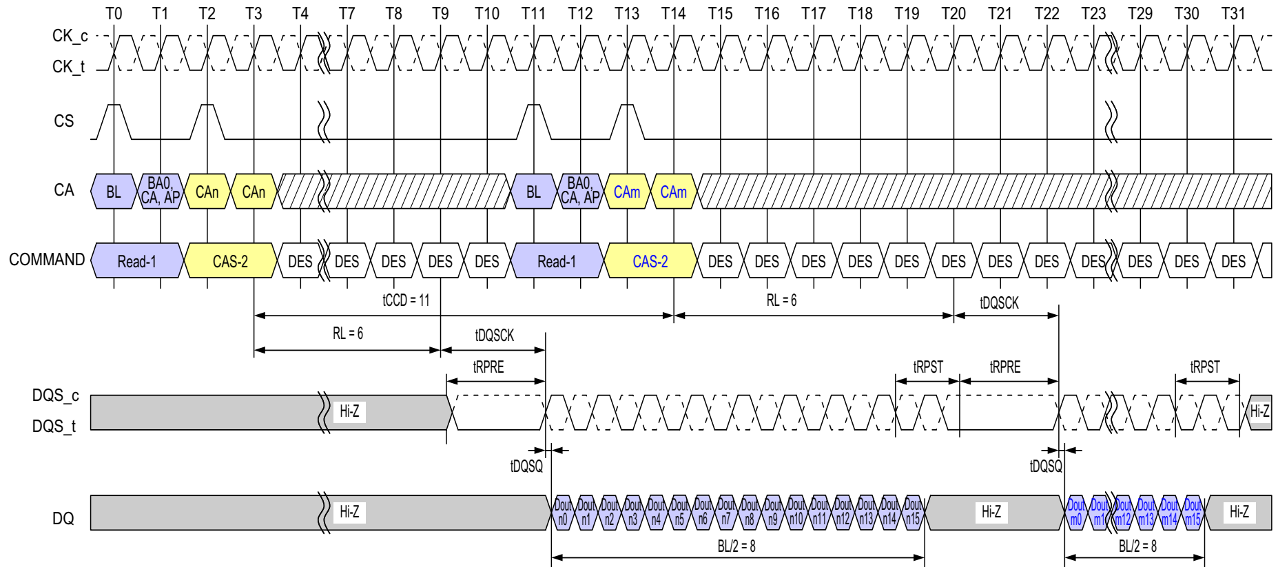
Figure 37 - Consecutive Reads Operation: tCCD = Min +3, Preamble = Static, 1.5nCK Postamble
