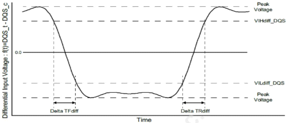
Figure 168 - Differential Input Slew Rate Definition for DQS t , DQS c
