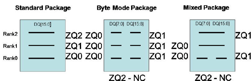
Figure 135 - ZQ Wiring Overview
