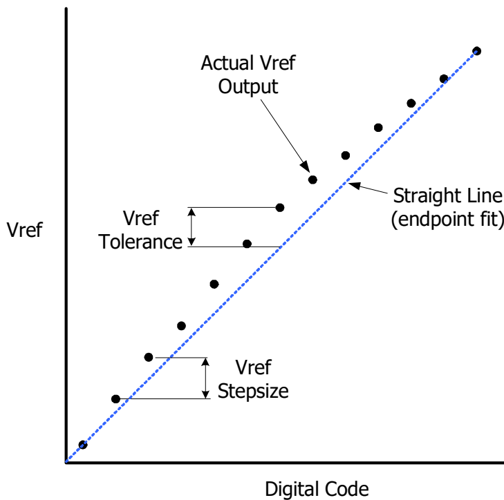
Figure 85 - Example of Vref set tolerance (max case only shown) and step size
