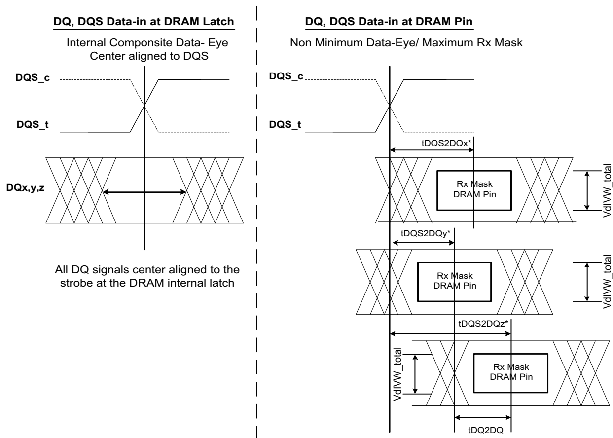
Figure 188 - DQ to DQS (tDQS2DQ and tDQDQ) Timings at the DRAM pins referenced from the internal latch
