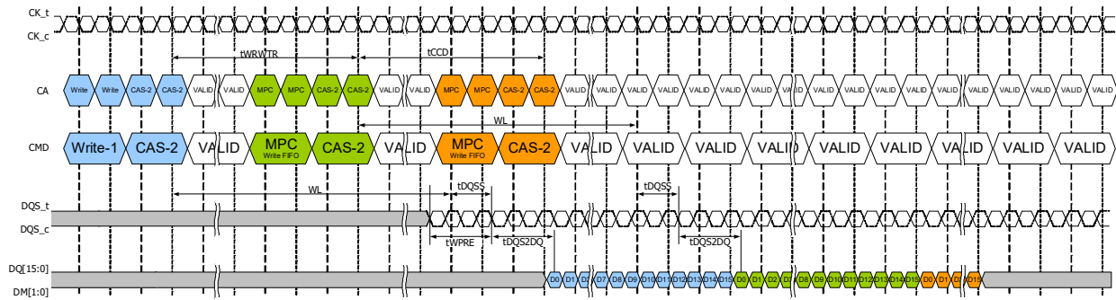
Figure 130 - MPC [WR FIFO] Operation :WPST = 2nCK, tWPST = 0.5nCK
