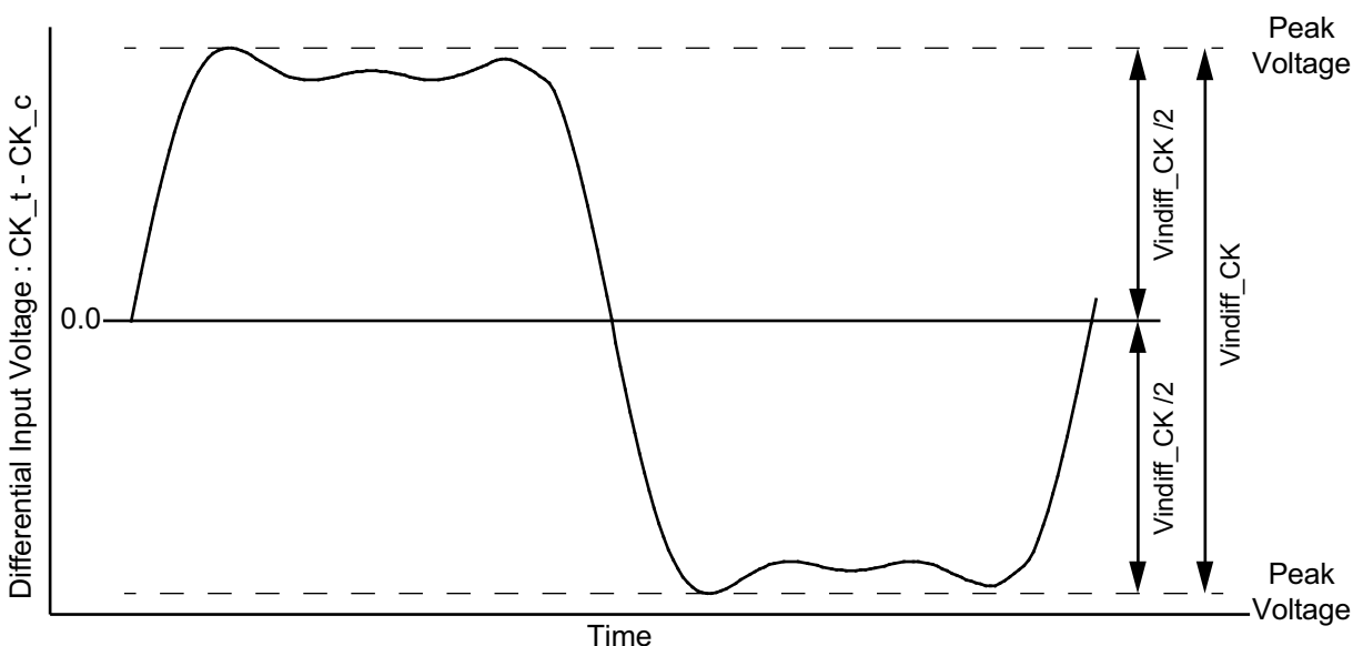
Figure 160 - CK Differential Input Voltage
