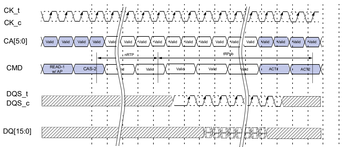
Figure 57 - Burst Read with Auto-Precharge (BL16, Toggling preamble)
