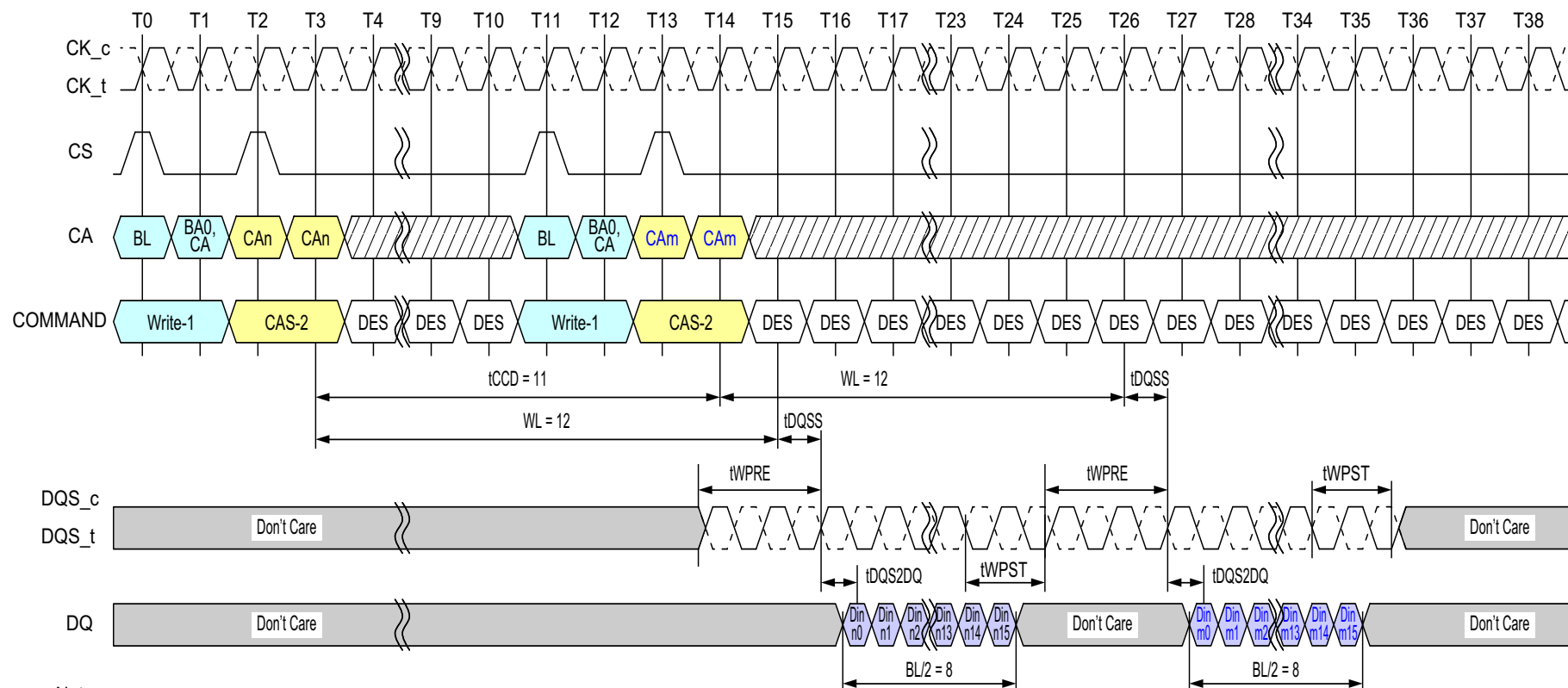
Figure 47 - Consecutive Writes Operation: t_{CCD} = \text{Min} + 3 , 1.5nCK Postamble
