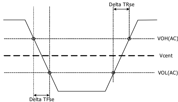
Figure 170 - Single Ended Output Slew Rate Definition
