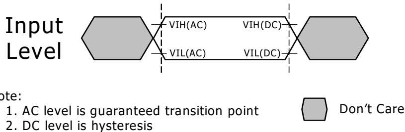
Figure 157 - Input AC timing definition for CKE
