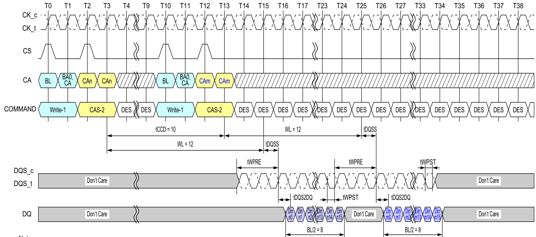
Figure 44 - Consecutive Writes Operation: t_{CCD} = \text{Min} + 2, 0.5nCK Postamble
