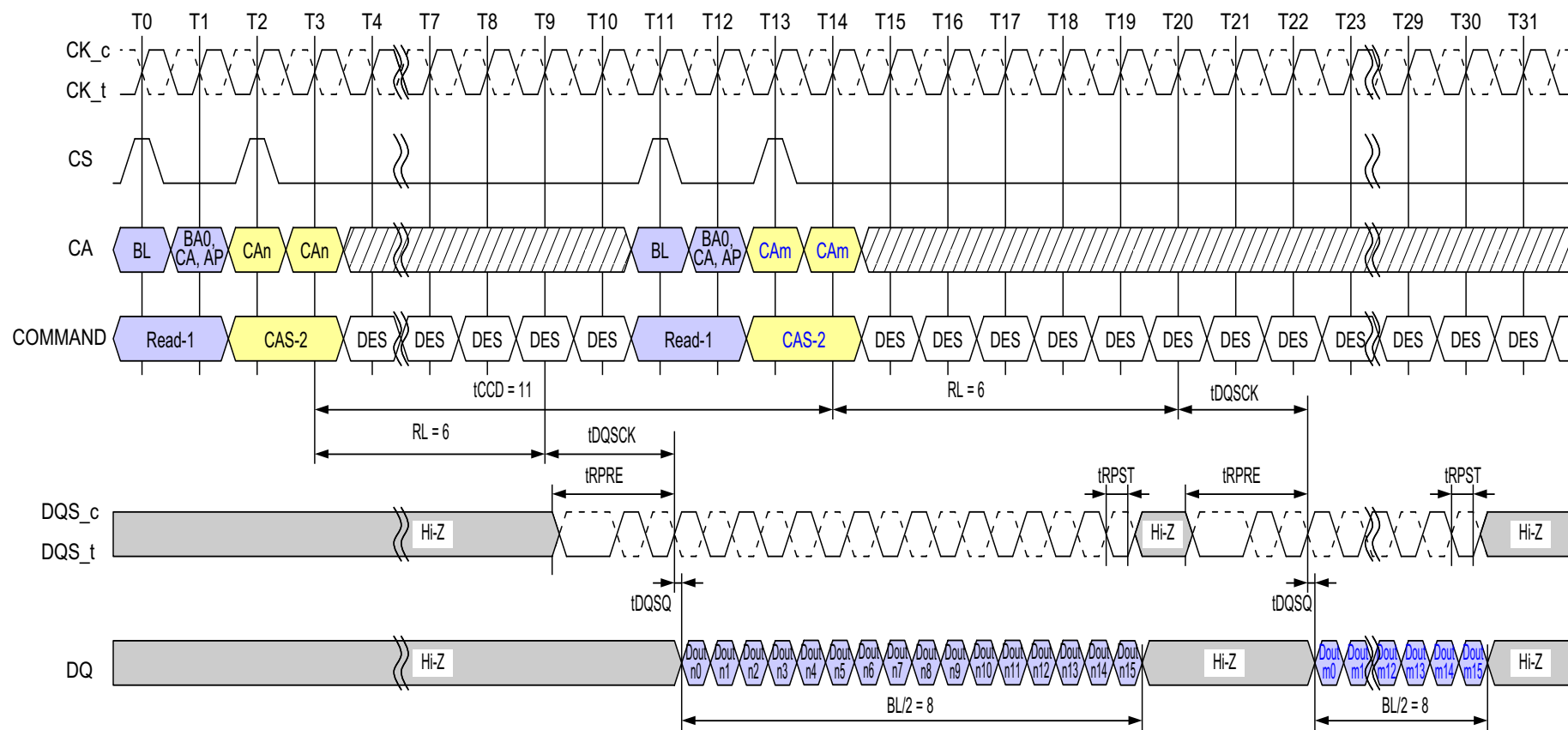
Figure 36 - Consecutive Reads Operation: t CCD = Min +3, Preamble = Toggle, 0.5nCK Postamble
