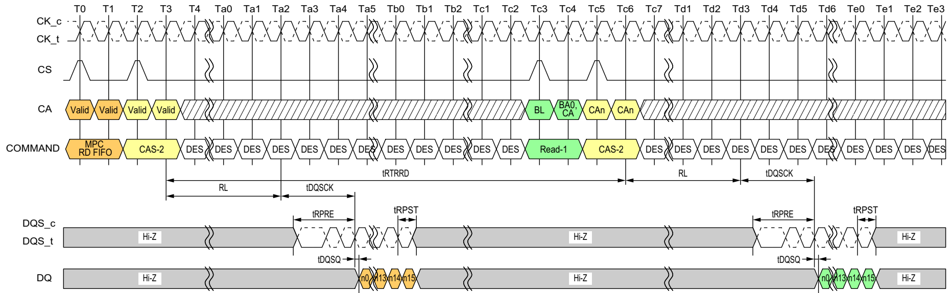
Figure 123 - MPC [Read FIFO] to Read Timing
