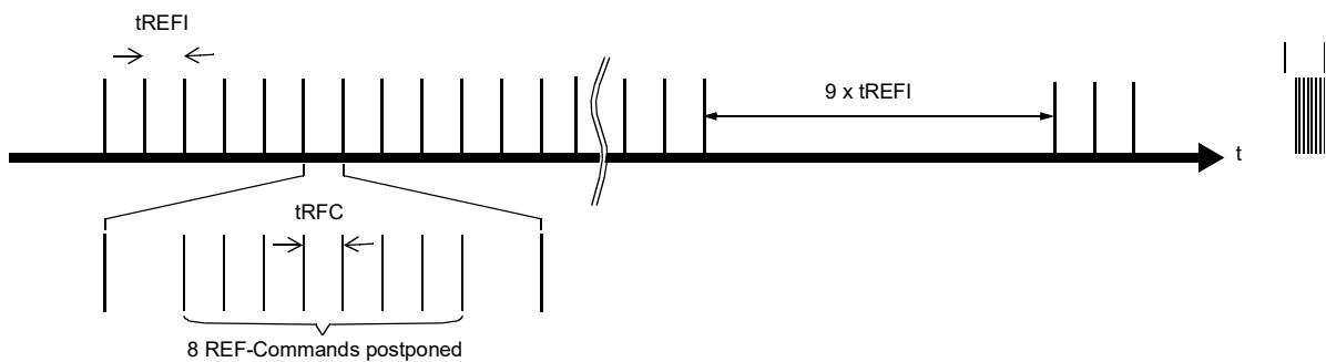
Figure 68 - Pulling-in Refresh Commands (Example)
