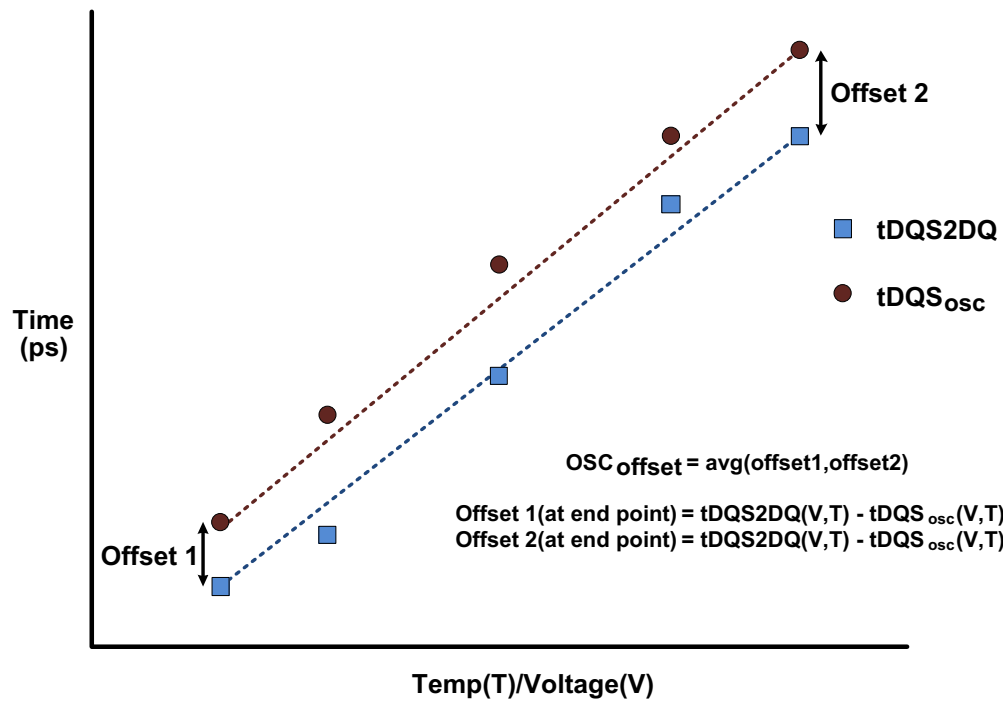
Figure 126 - Interval oscillator offset (OSC offset )
