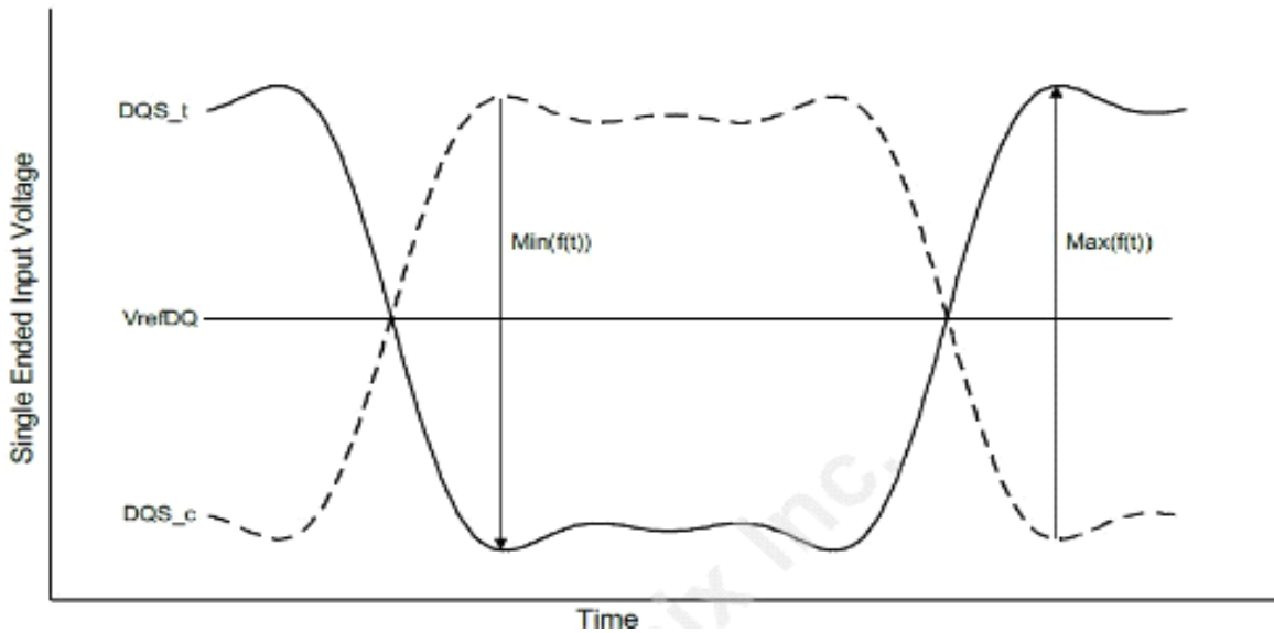
Figure 166 - Definition of differential DQS Peak Voltage
