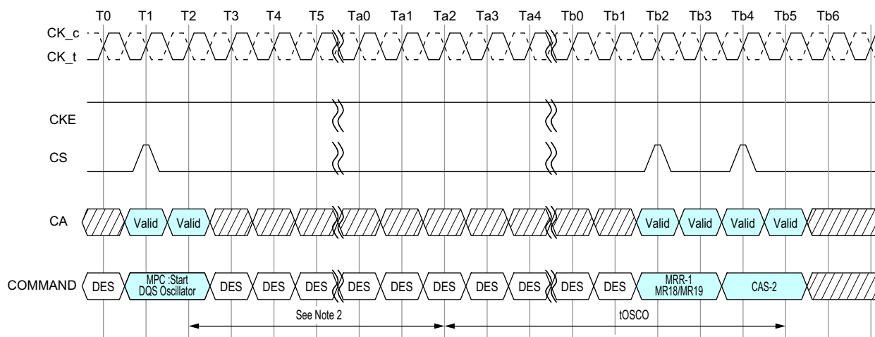
Figure 128 - In case of DQS Interval Oscillator is stopped by DQS interval timer
