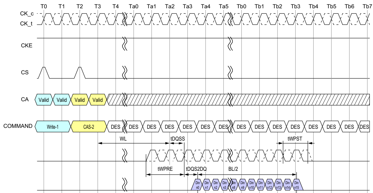
Figure 20 - DQS Write Preamble and Postamble: 1.5nCK Postamble
