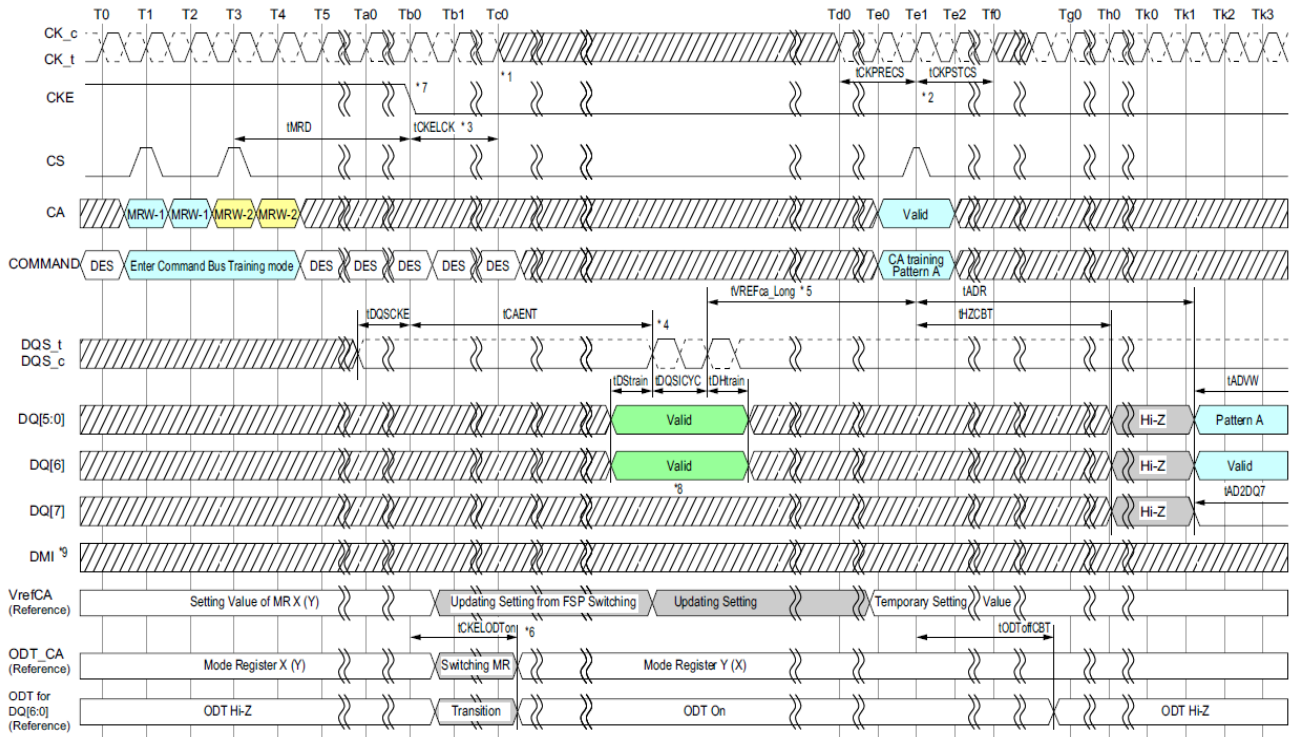
Figure 105 - Entering CBT mode and CA Training Pattern Input with VREFCA Value Update
