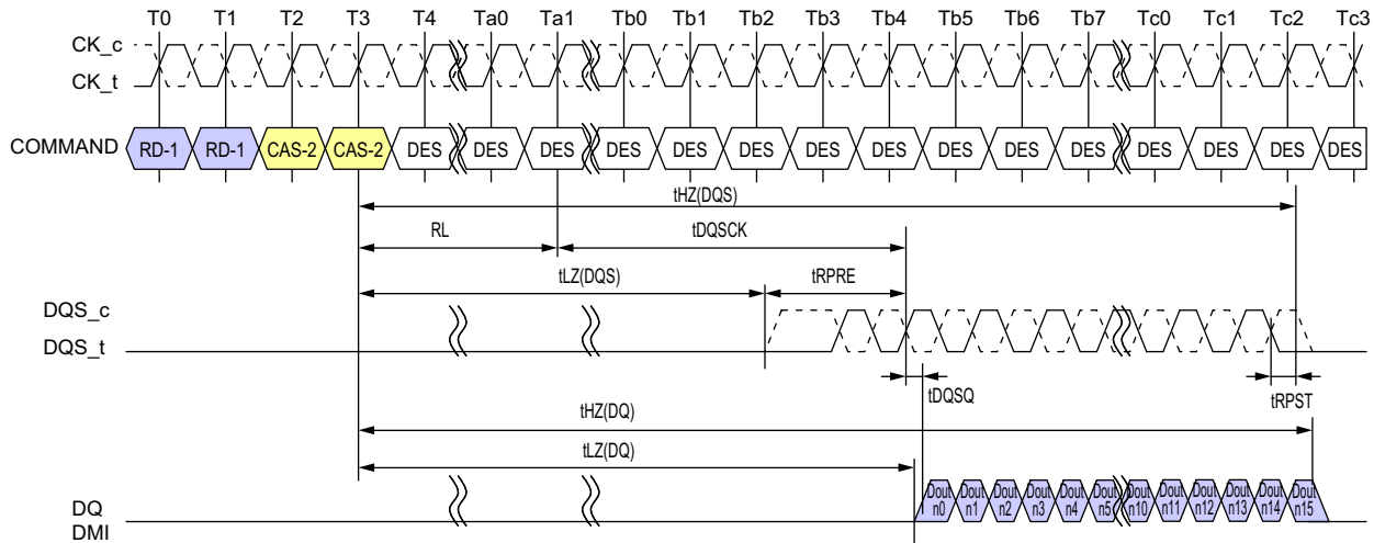
Figure 11 - Read Timing
