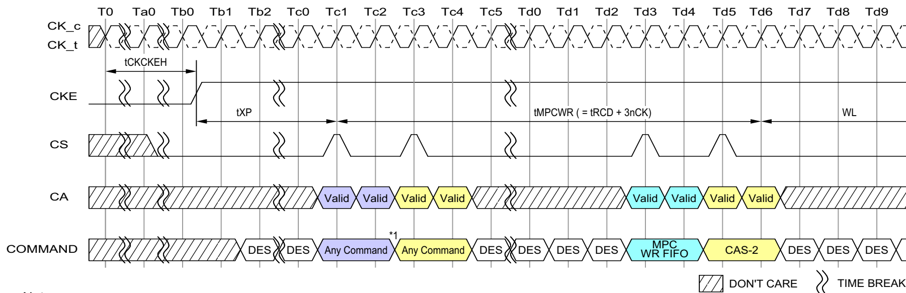
Figure 125 - Power Down Exit to MPC [Write FIFO] Timing
