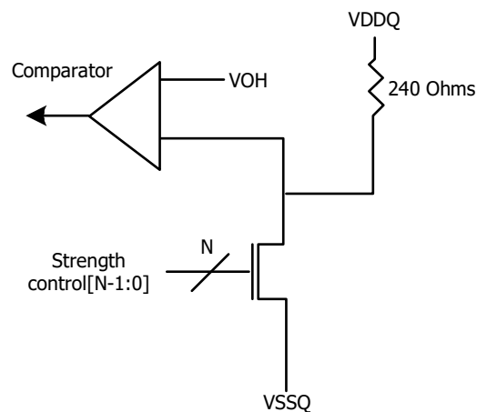
Figure 175 - Pull-down calibration
