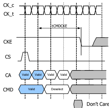
Figure 178 - tCMDCKE Timing
