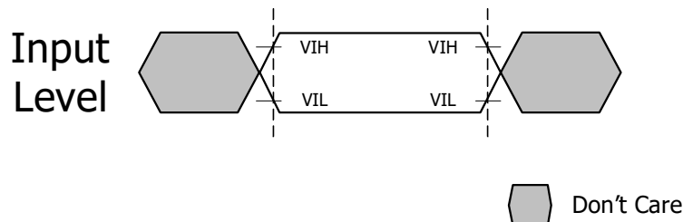
Figure 158 - Input AC timing definition for Reset_n and ODT_CA
