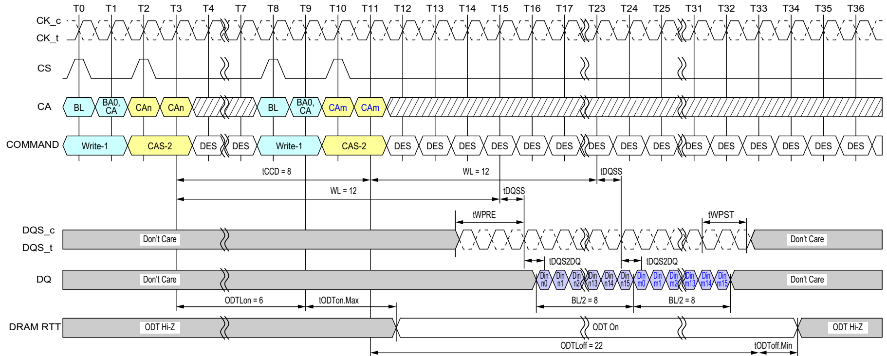
Figure 40 - Seamless Writes Operation: t_{CCD} = \text{Min}, 1.5nCK Postamble, 533\text{MHz} < \text{Clock Freq.} \leq 800\text{MHz} , ODT Worst Timing Case
