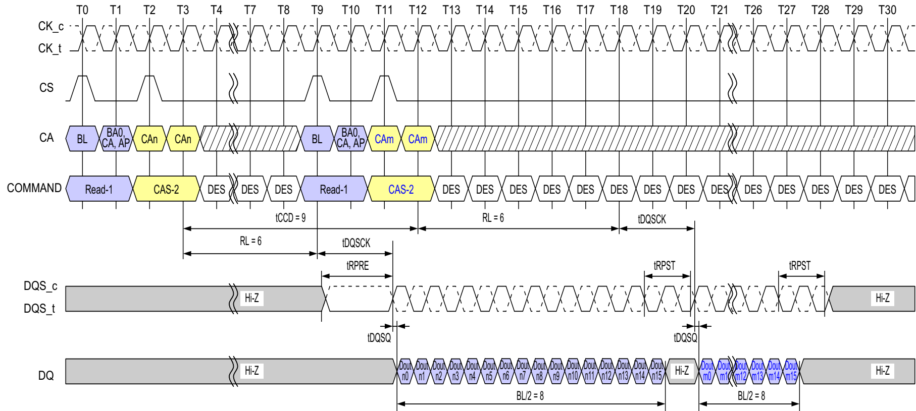
Figure 29 - Consecutive Reads Operation: tCCD = Min + 1, Preamble = Static, 1.5nCK Postamble
