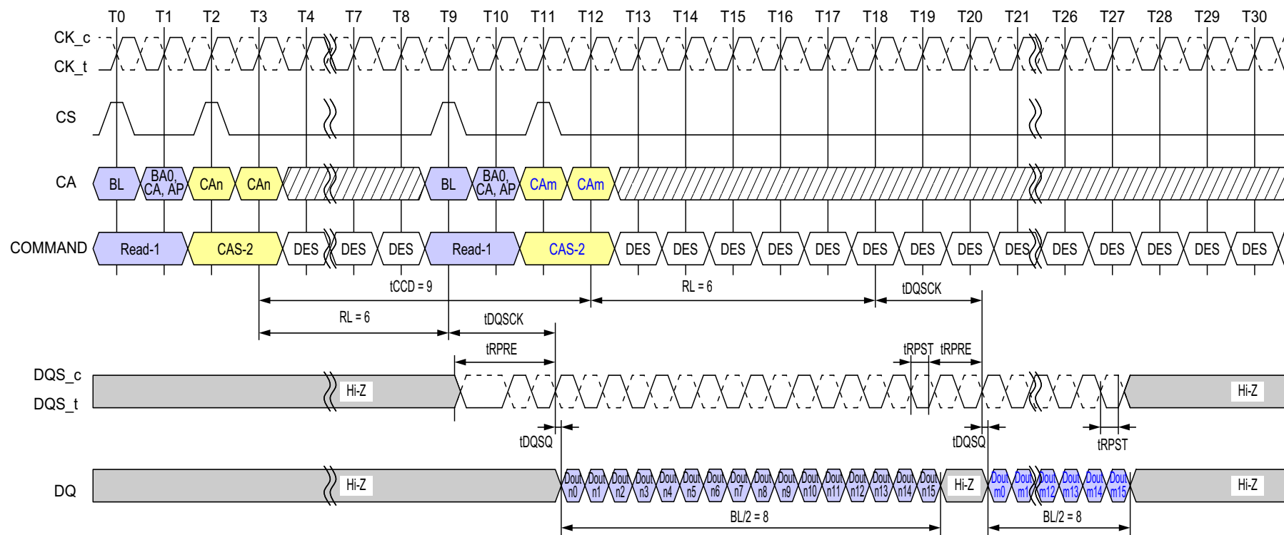
Figure 28 - Consecutive Reads Operation: t_{CCD} = \text{Min} + 1 , Preamble = Toggle, 0.5nCK Postamble
