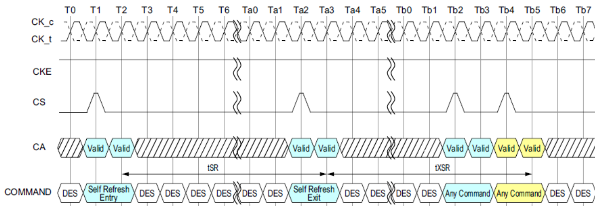
Figure 72 - Self Refresh Entry/Exit Timing
