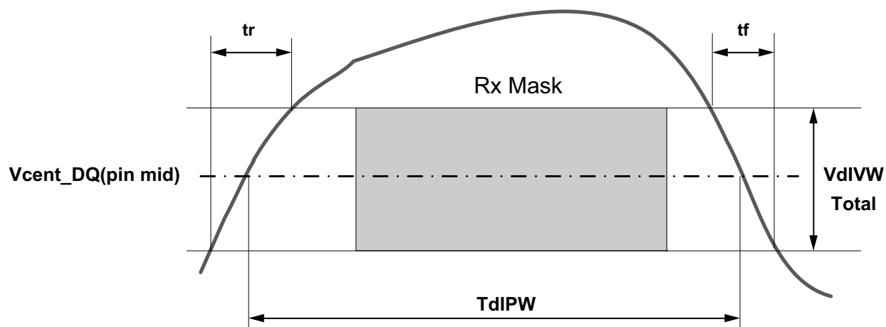
Figure 189 - DQ TdIPW and SRIN_dIVW definition (for each input pulse)
