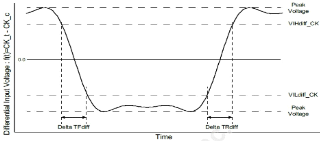
Figure 163 - Differential Input Slew Rate Definition for CK_t, CK_c
