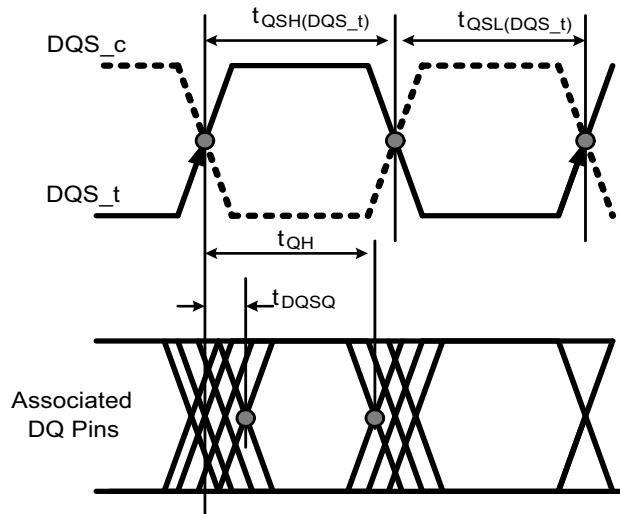
Figure 184 - Read data timing definitions t_{QH} and t_{DQSQ} across on DQ signals per DQS group
