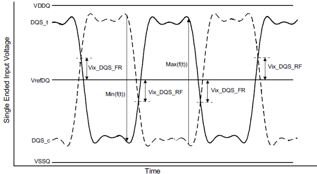
Figure 169 - Vix Definition (DQS)
