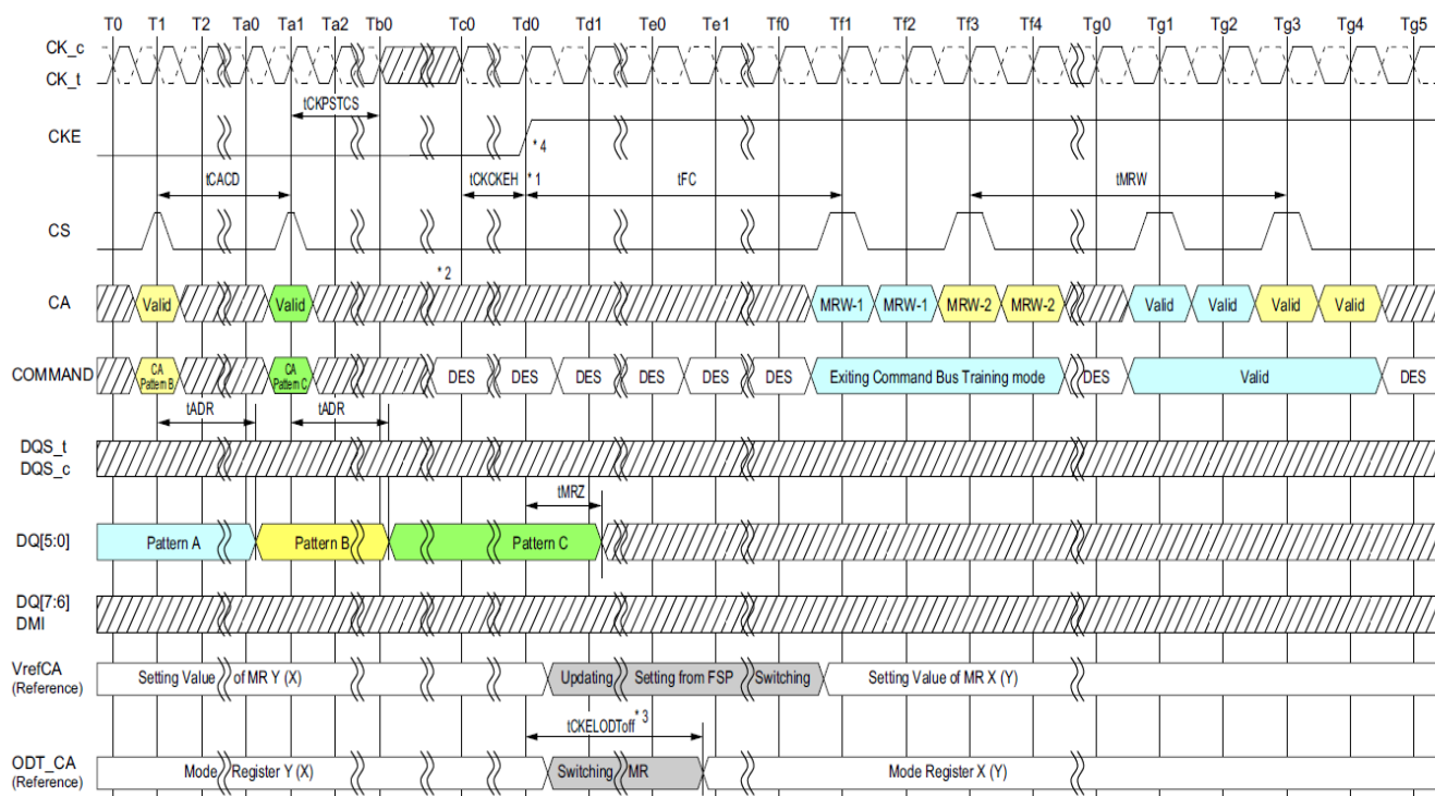
Figure 103 - Exiting Command Bus Training Mode with Valid Command
