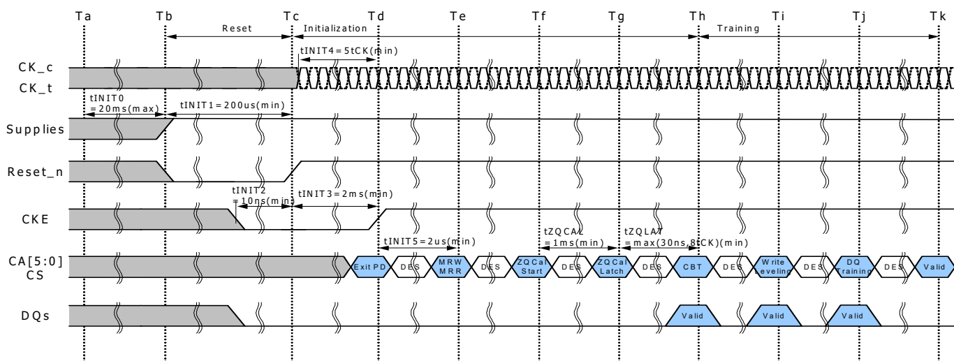
Figure 3 - Power Ramp and Initialization Sequence
