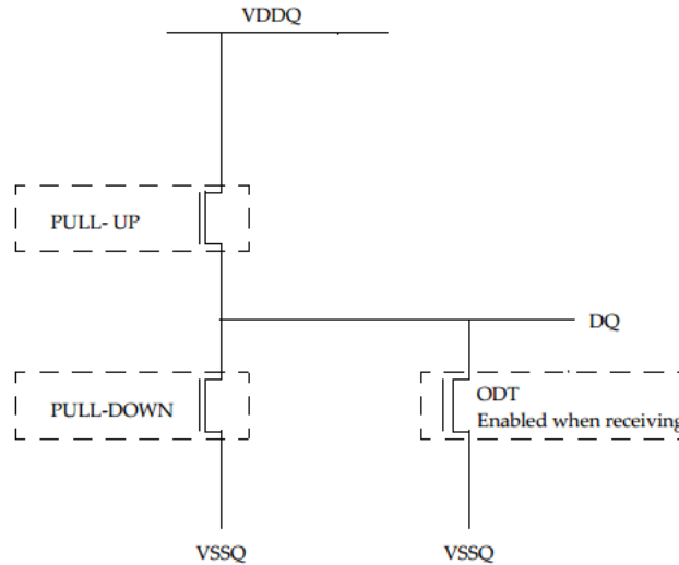
Figure 174 - LVSTL I/O Cell
