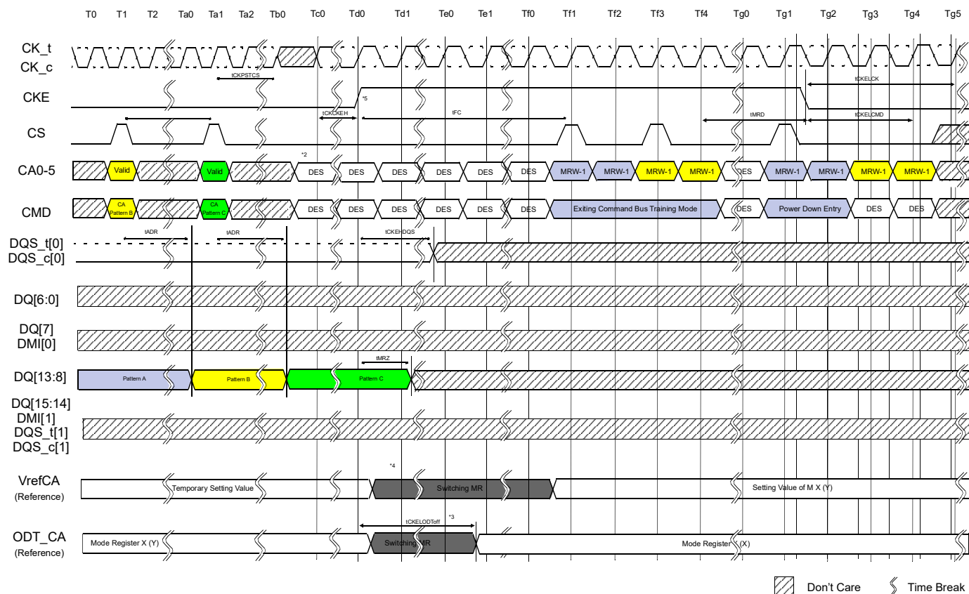
Figure 101 - Exiting Command Bus Training Mode with Power Down Entry
