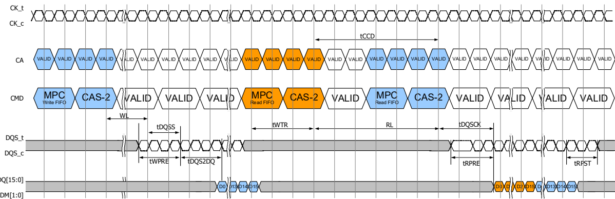
Figure 131 - MPC [RD FIFO] Read Operation (Shown with tWPST=2nCK, tWPST=0.5nCK, tRPST=toggling, tRPST=1.5nCK)
