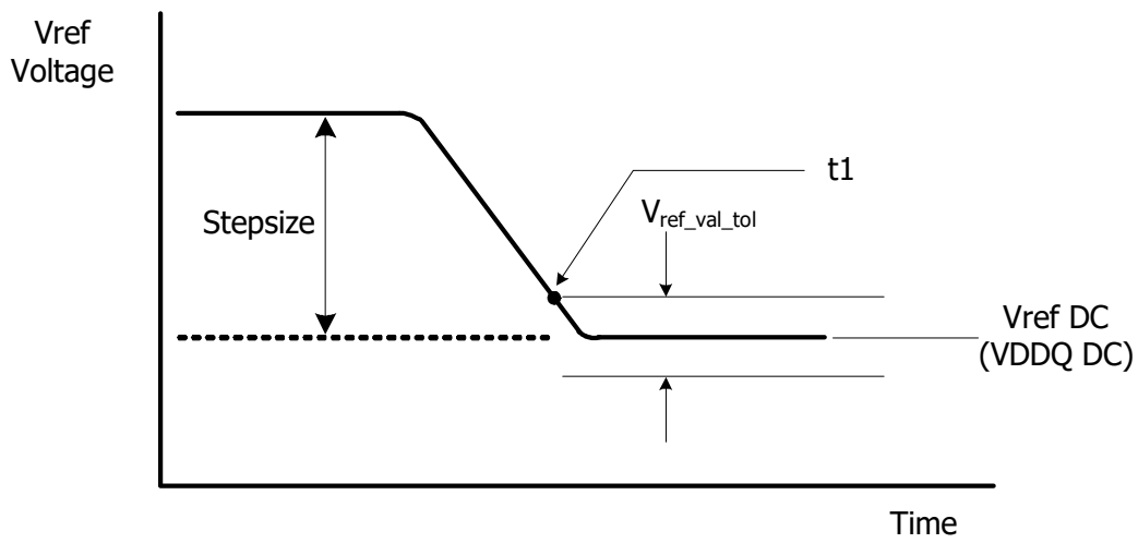
Figure 95 - Vref step single step size decrement case
