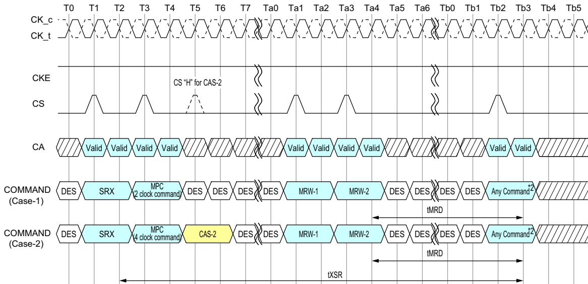
Figure 75 - MRR, MRW and MPC Commands Issuing Timing during tXSR
