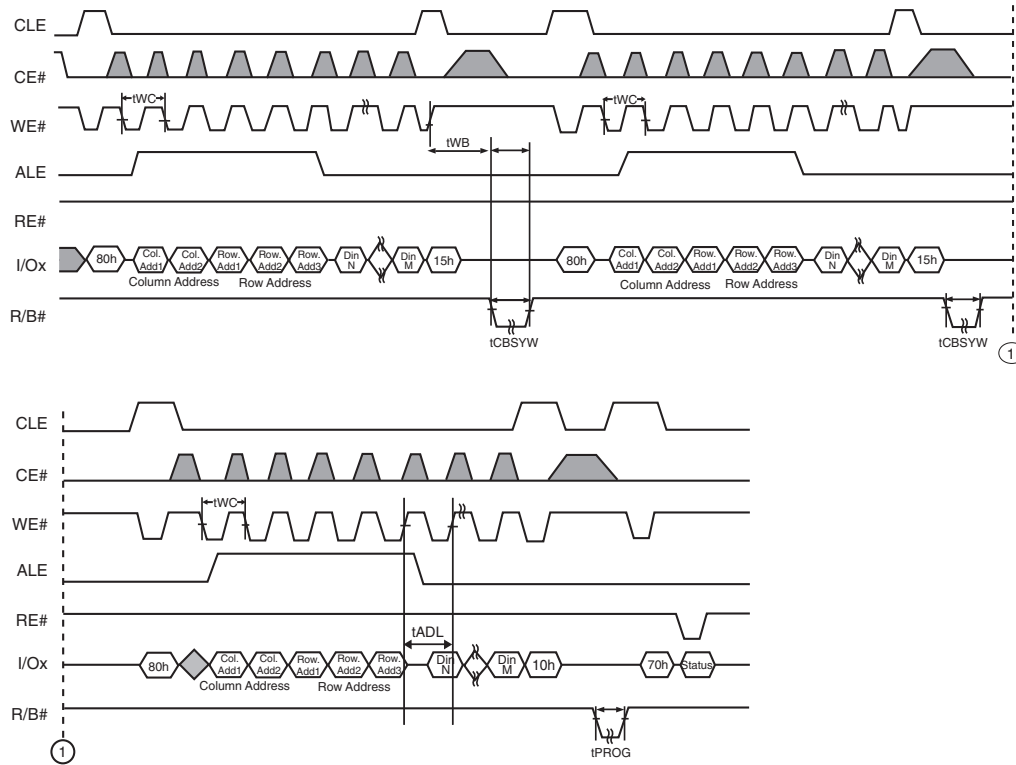
Figure 6.23 Cache Program
