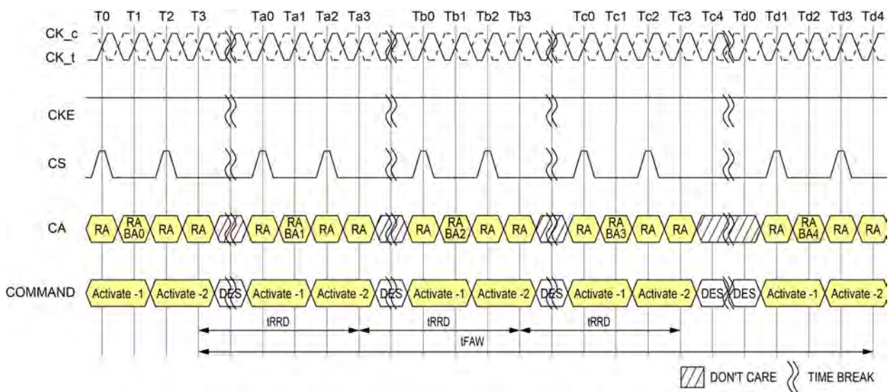
Figure 5 - tFAW Timing
