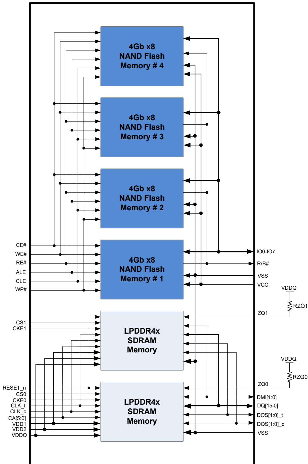
Figure 2.1 Block Diagram
