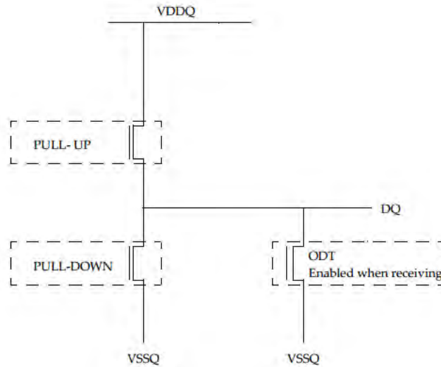
Figure 185 - LVSTL I/O Cell
