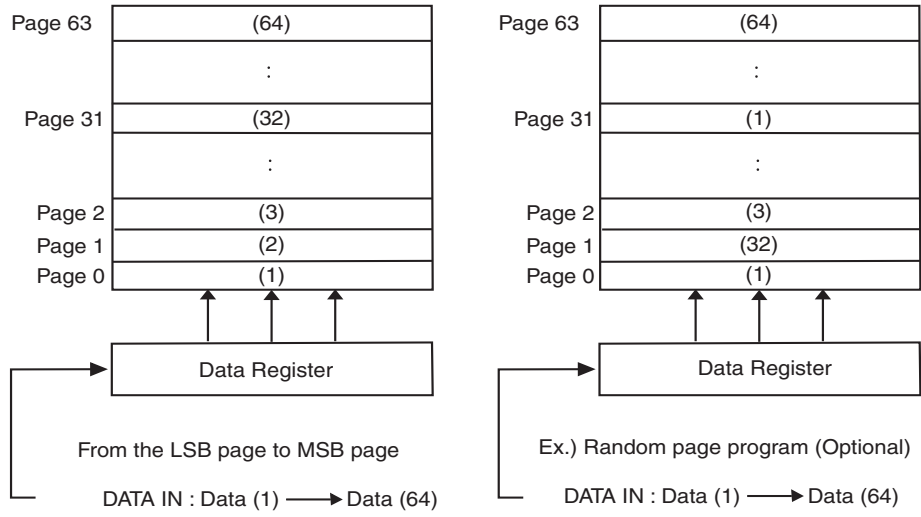
Figure 8.3 Page Programming Within a Block
