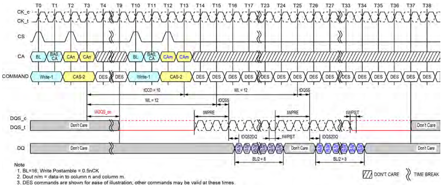
Figure 47 - Consecutive Writes Operation: t CCD = Min + 2, 0.5nCK Postamble
