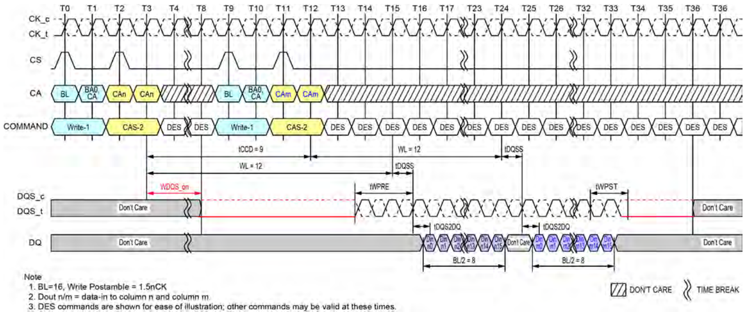
Figure 46 - Consecutive Writes Operation: t CCD = Min + 1, 1.5nCK Postamble
