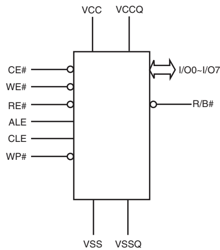
Figure 1.1 Logic Diagram
