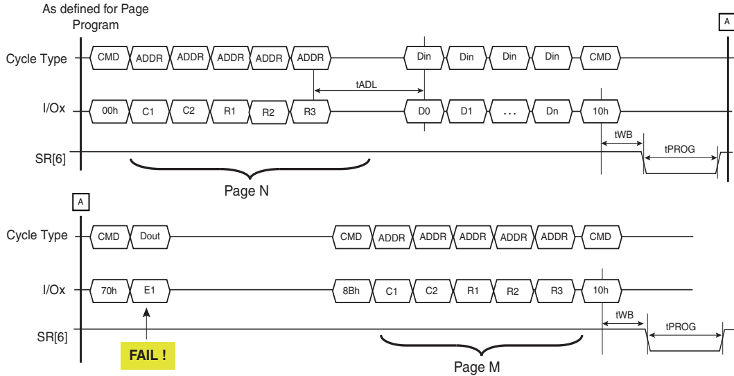
Figure 3.1 Page Reprogram
